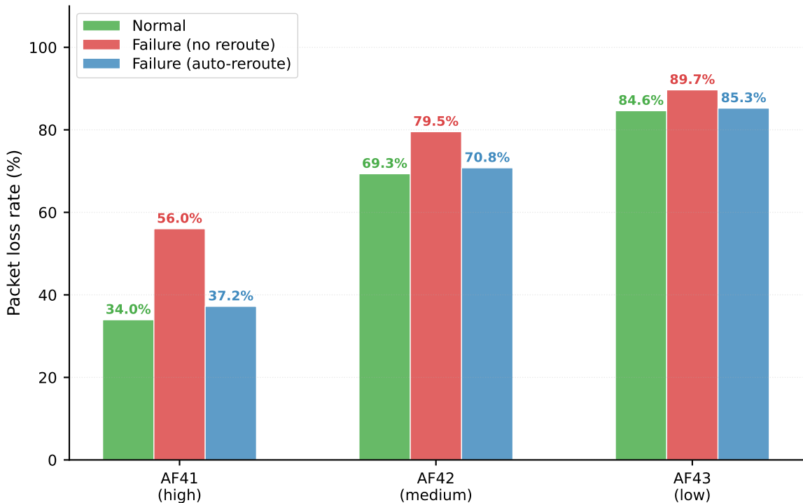
UDP packet loss rate (iperf3 measured, 60 s average)
