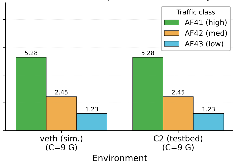
SP disabled (WRR quantum ratio 4:2:1 only)
