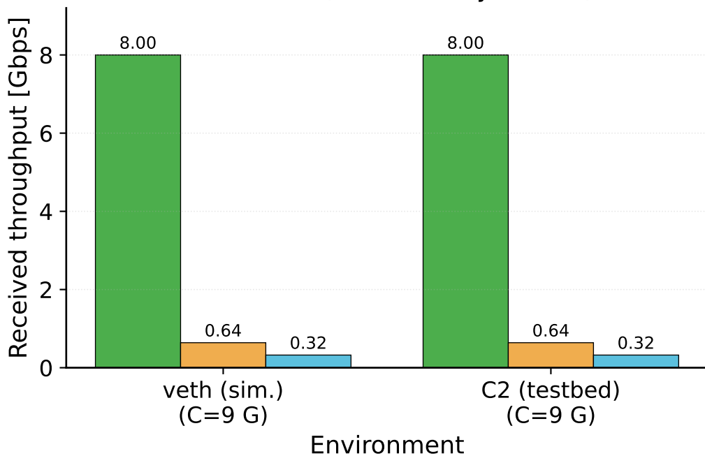
SP enabled (Strict Priority + WRR)
