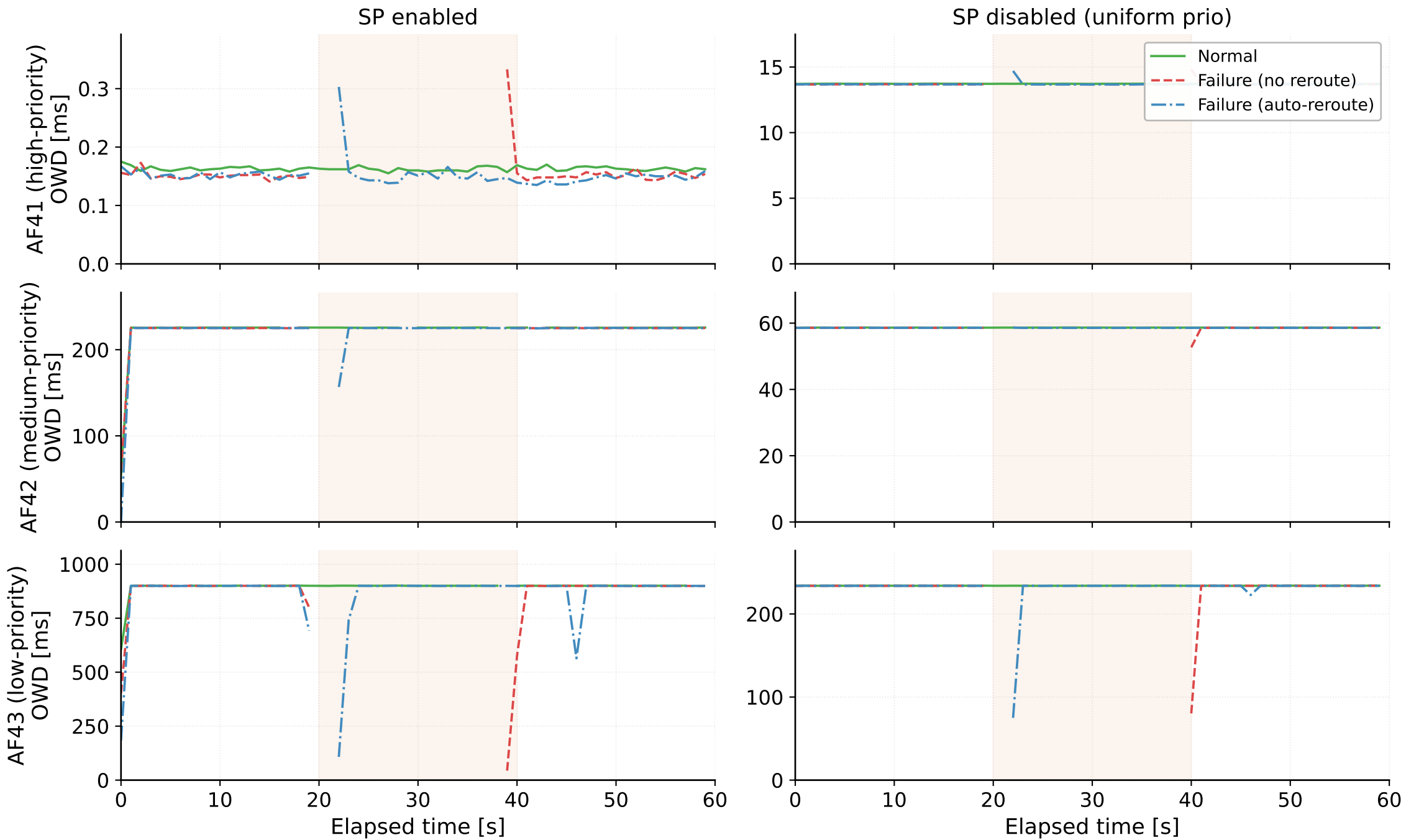
Per-scenario One-Way Delay — SP enabled vs disabled (C2(testbed) (C=9 G), failure window t=20-40 s, 1 s median)
