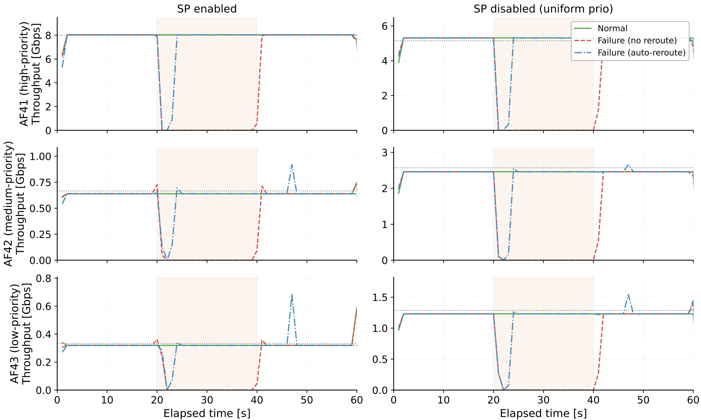
Per-scenario Throughput — SP enabled vs disabled (C2 (testbed) (C=9 G), failure window t=20–40 s shaded)
