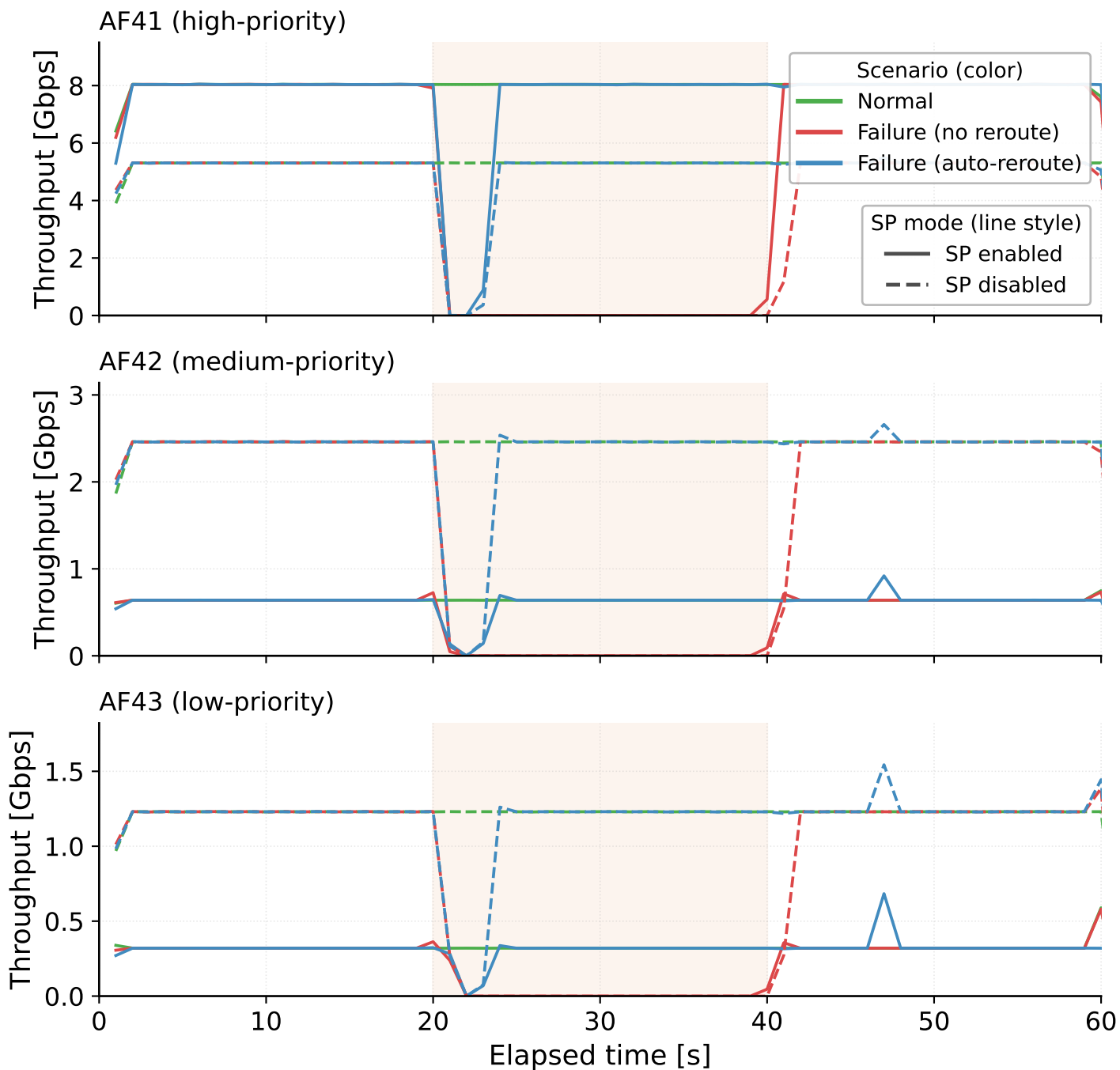
Received Throughput — SP enabled/disabled overlaid on shared axis (C2 (testbed) (C=9 G), failure window t=20-40 s shaded)
