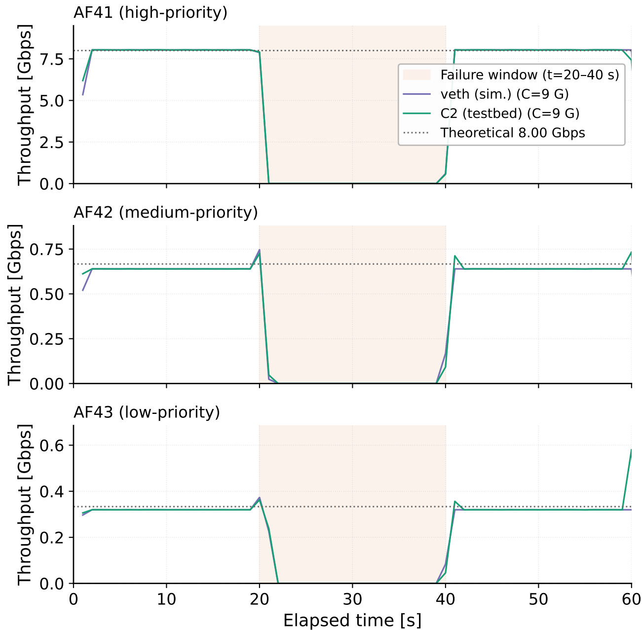
Received Throughput over Time: Simulation (veth) vs Hardware (C2) (SP enabled, failure (no reroute))
