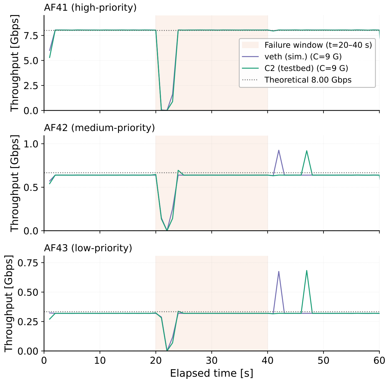
Received Throughput over Time: Simulation (veth) vs Hardware (C2) (SP enabled, failure (auto-reroute))
