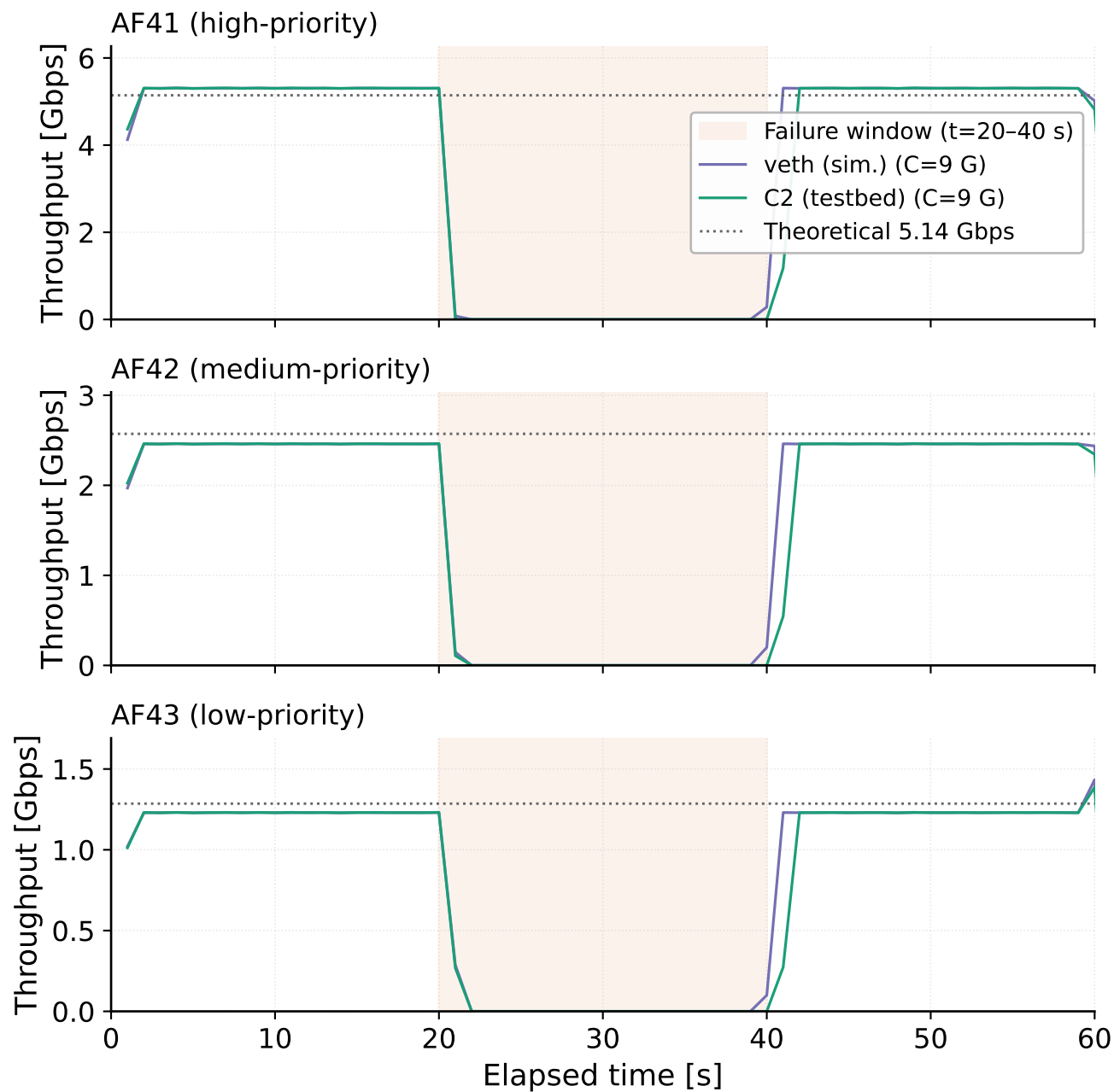
Received Throughput over Time: Simulation (veth) vs Hardware (C2) (SP disabled (uniform prio), failure (no reroute))
