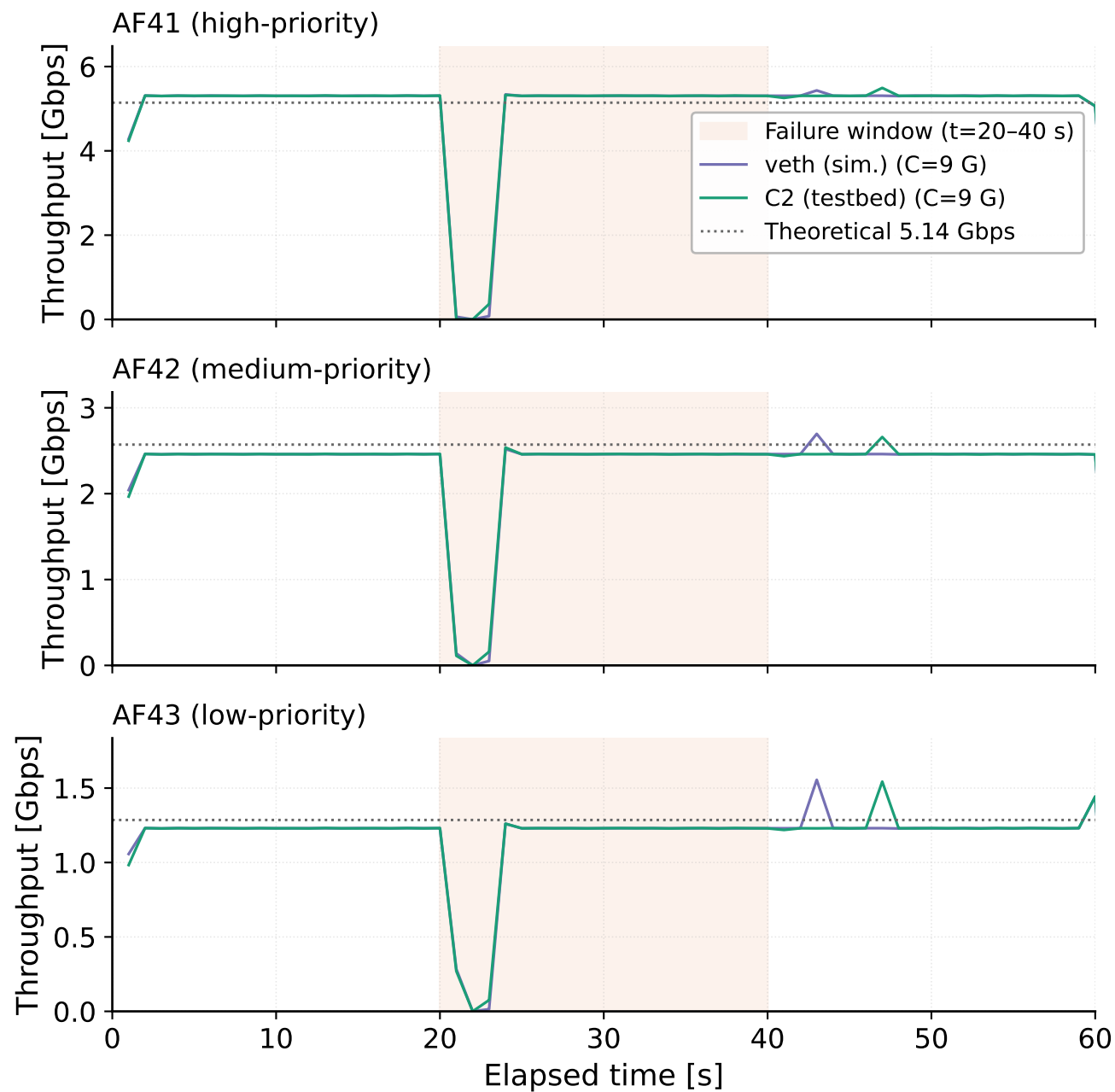
Received Throughput over Time: Simulation (veth) vs Hardware (C2) (SP disabled (uniform prio), failure (auto-reroute))
