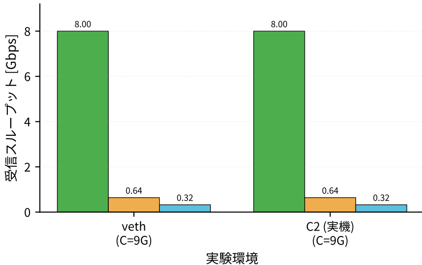
SP有効 (Strict Priority + WRR)
