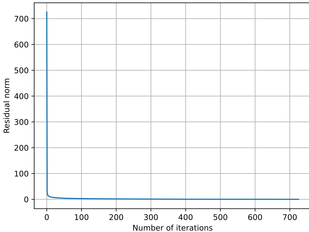
Residual Error of the GMRES Method
