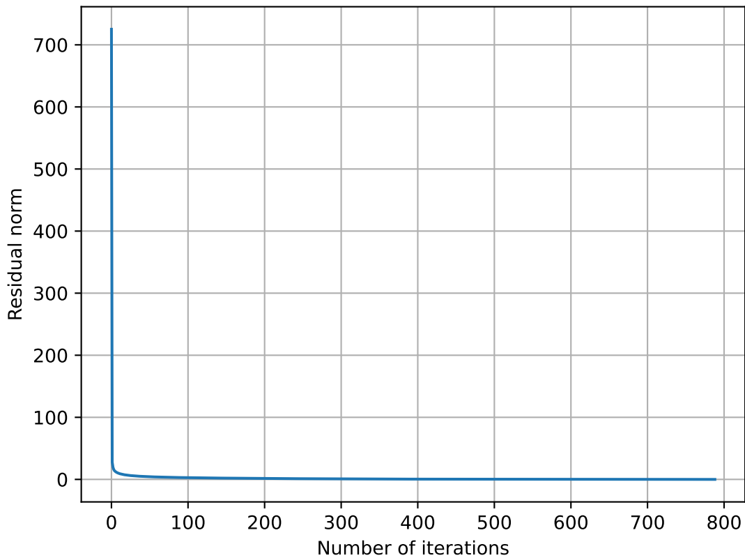
Residual Error of the Givens Rotation Method
