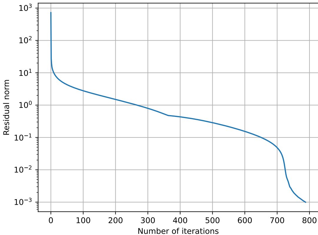
Residual Error of the Givens Rotation Method
