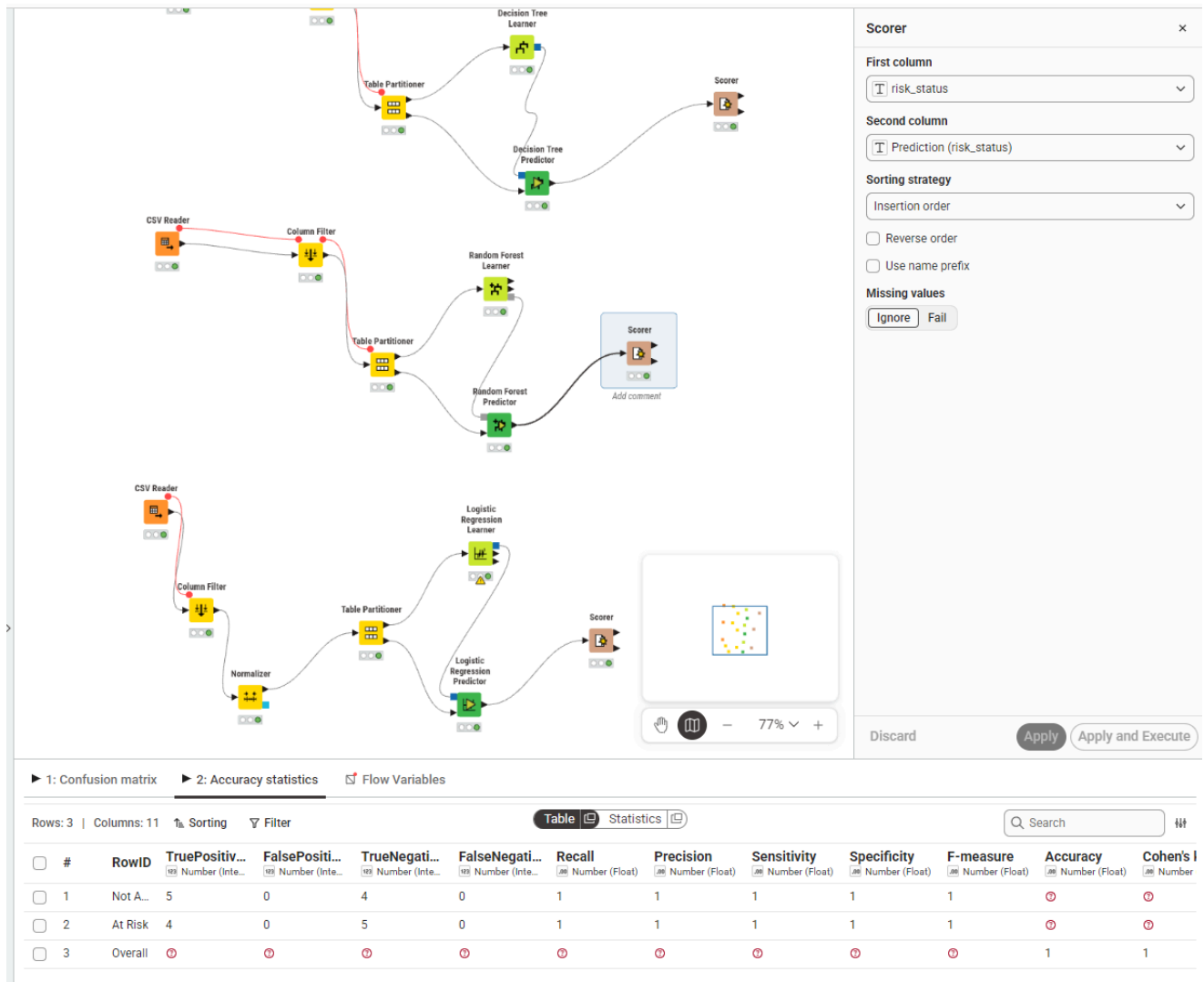
Random Forest evaluation results
