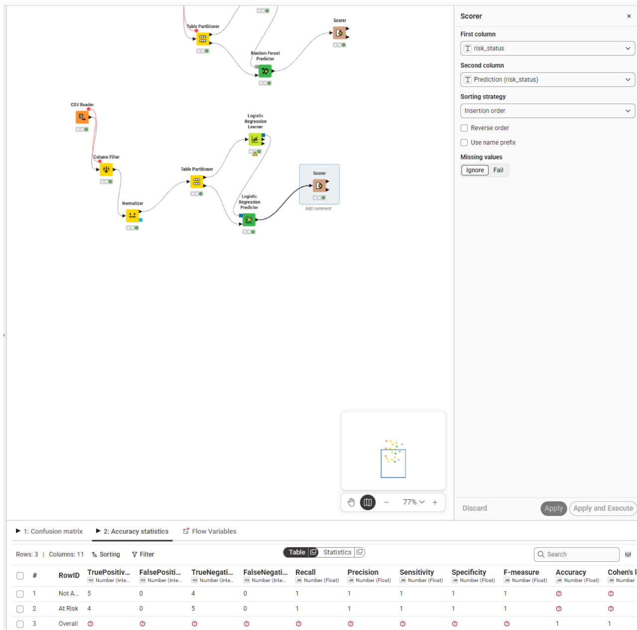
Logistic Regression evaluation results
