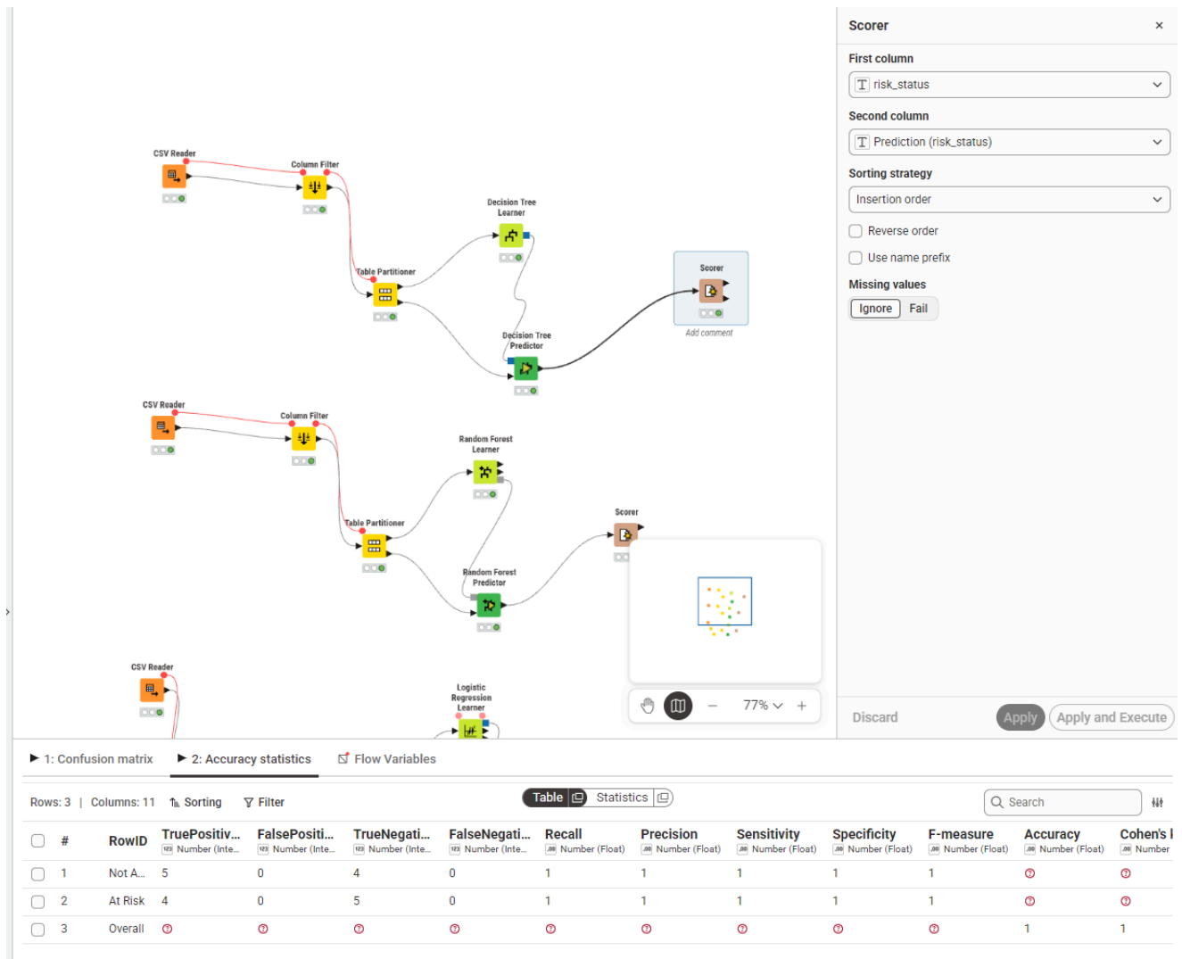
Decision Tree evaluation results
