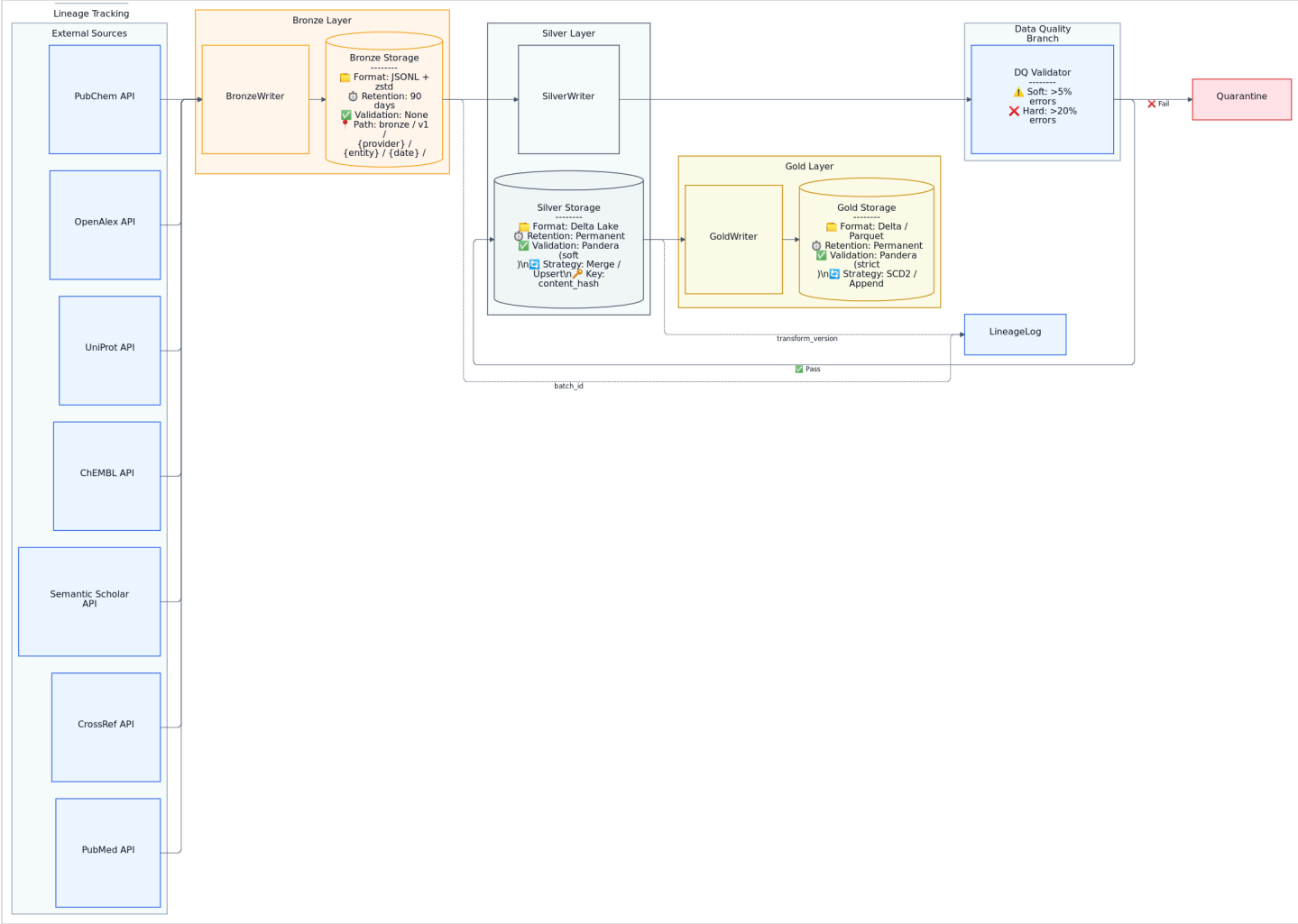
003. foundation/png/02-full-medallion-data-flow.png
