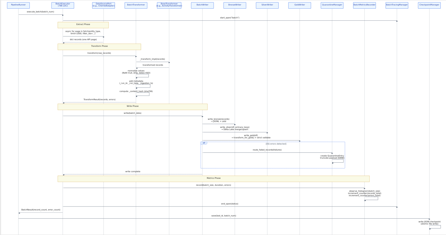
040. foundation/png/34-batch-processing-flow.png
