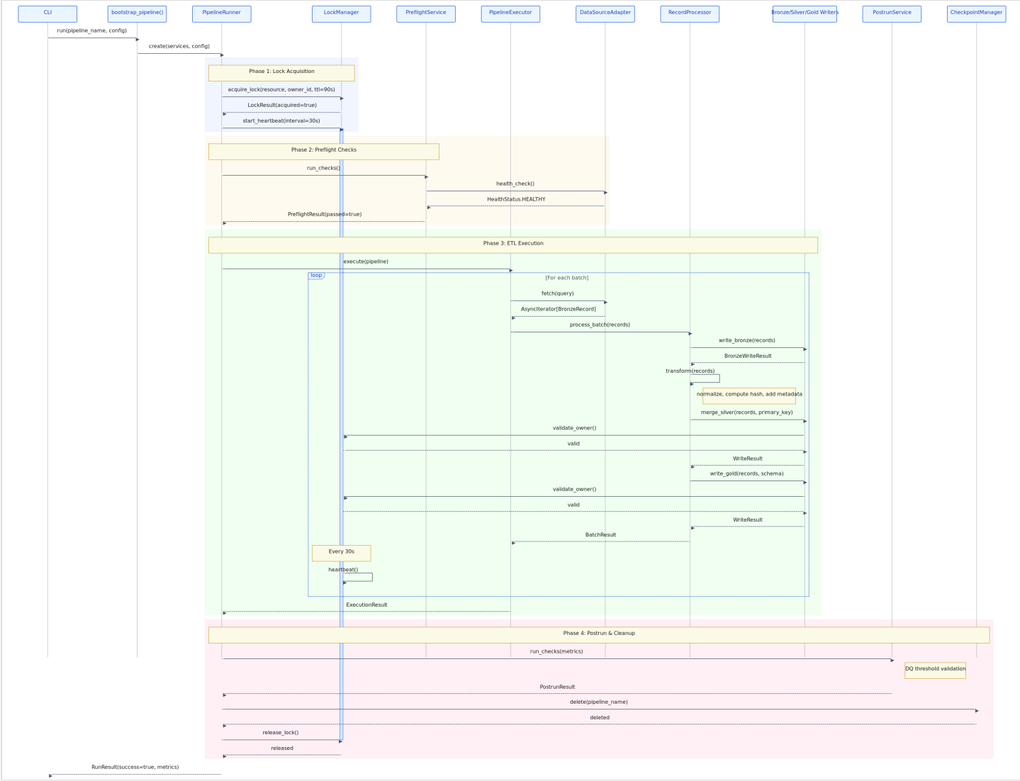
004. foundation/png/03-pipeline-execution-happy-path.png
