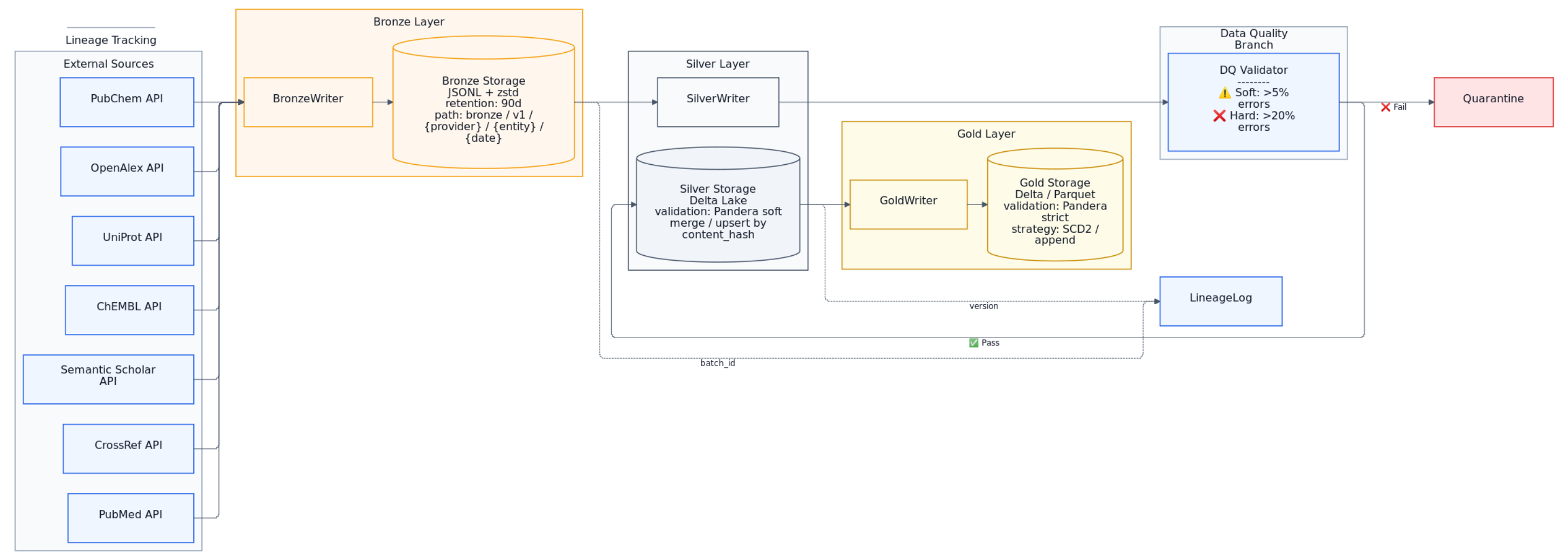
02-full-medallion-data-flow
