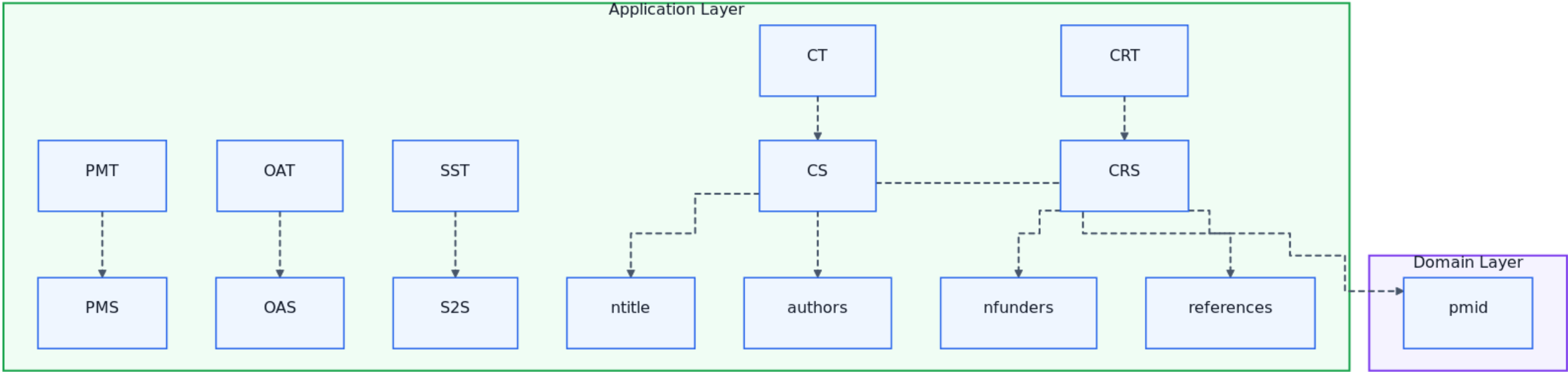
44-cross-provider-enrichment-overview
