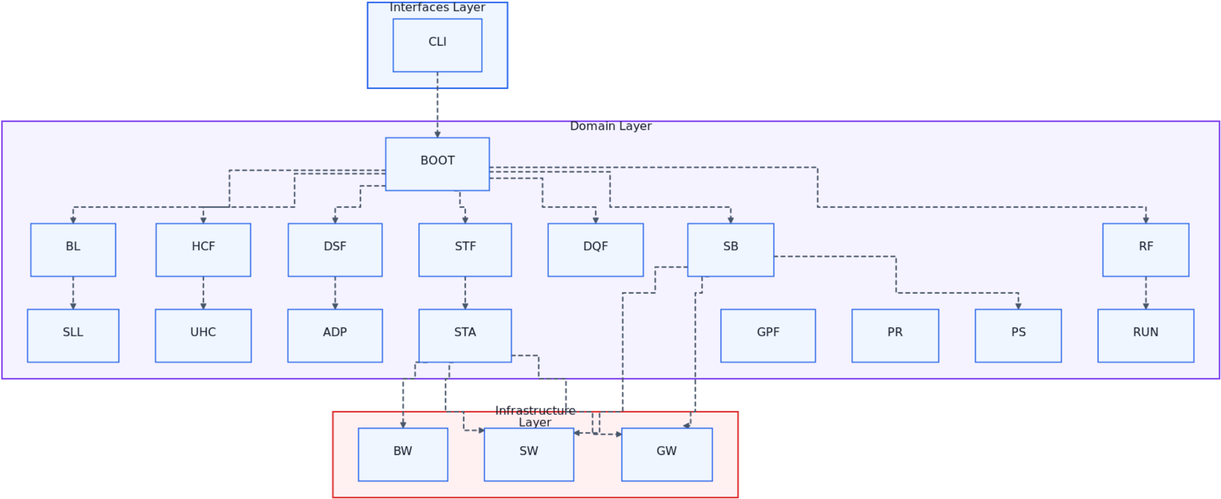
28-composition-root-di-graph-domain
