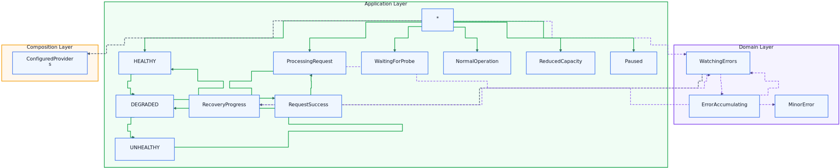
14-provider-health-states-overview
