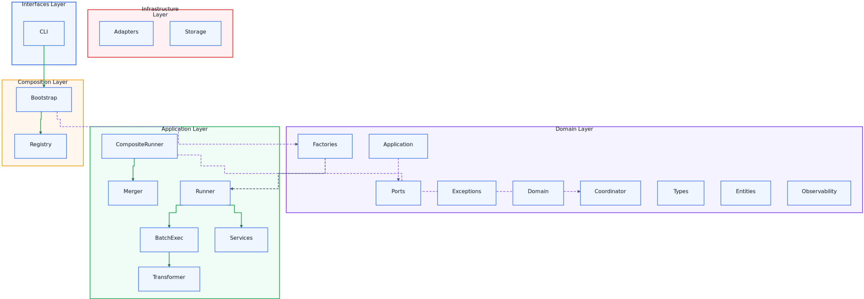
05-layers-interaction-domain
