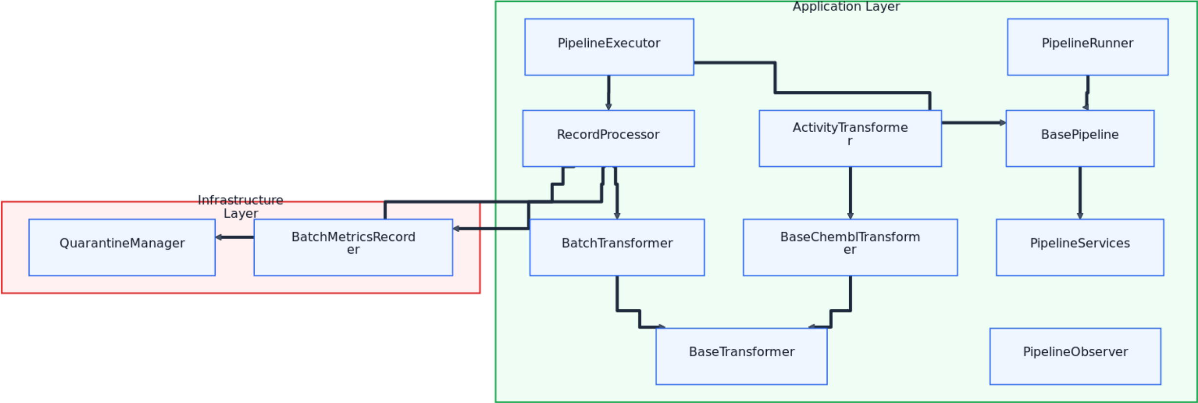
06-application-layer-class-diagram-dataflow
