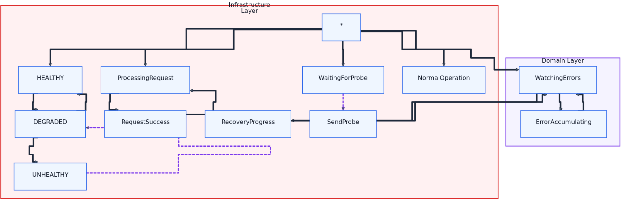
14-provider-health-states-dataflow
