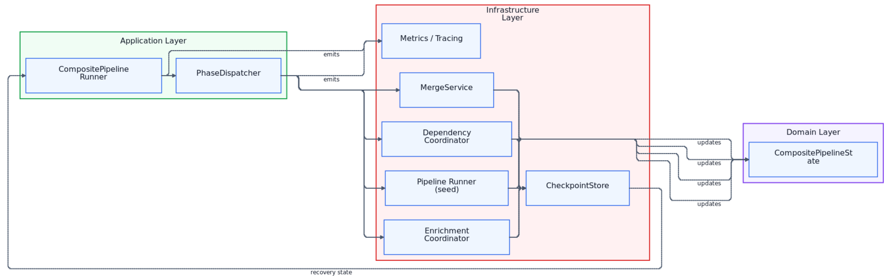
48-composite-phase-lifecycle-infra
