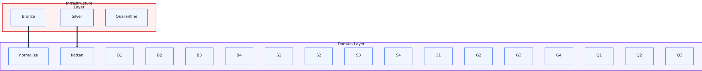
02-medallion-domain
