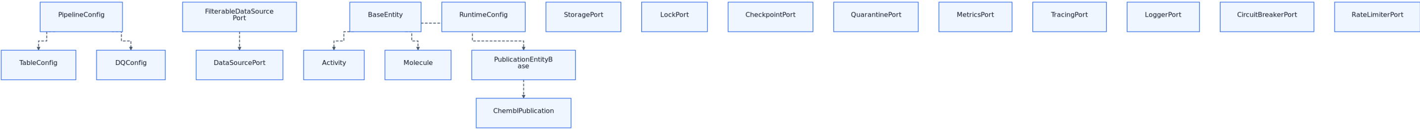
04-domain-layer-class-diagram-domain
