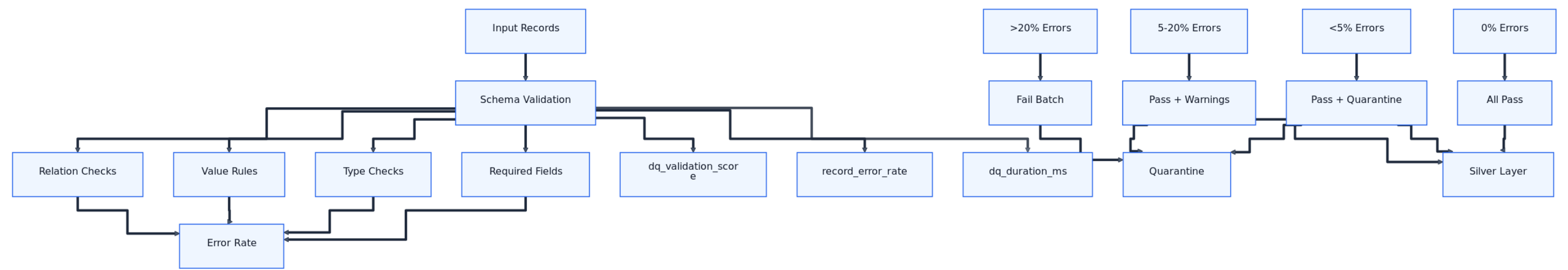
15-dq-check-workflow-domain
