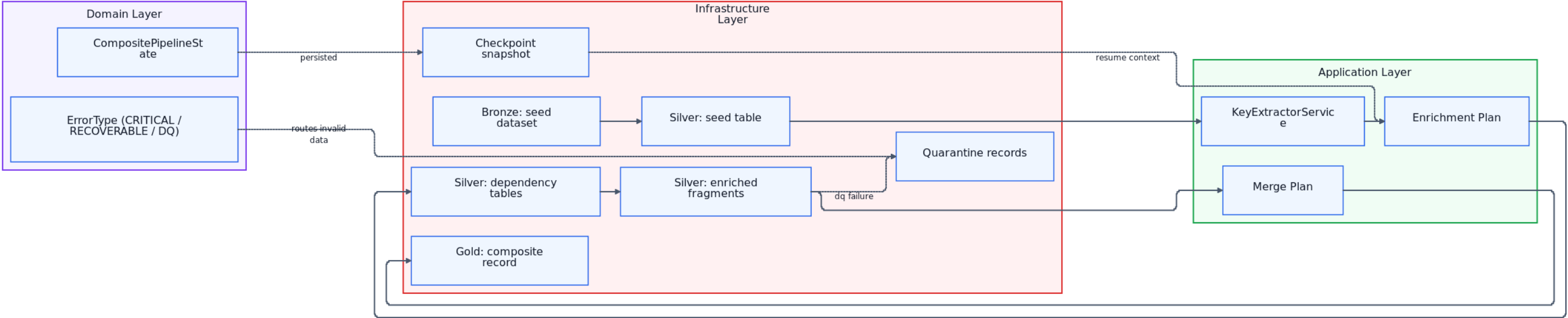
48-composite-phase-lifecycle-dataflow
