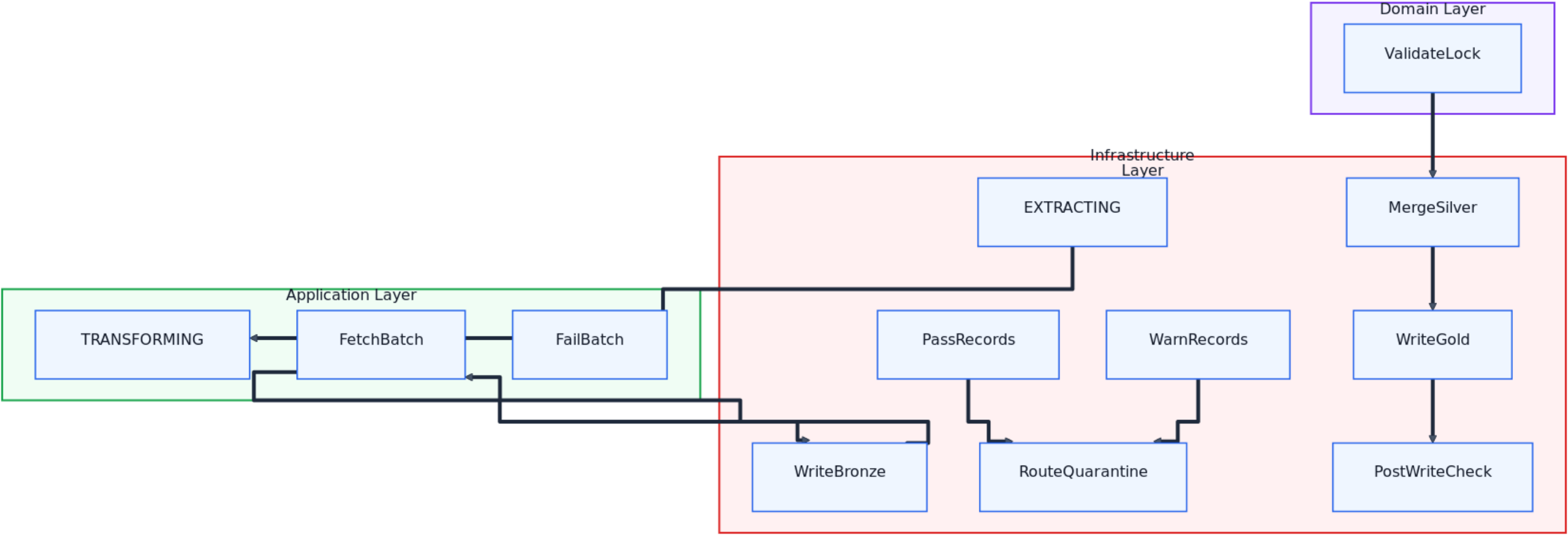
05-pipeline-lifecycle-states-dataflow
