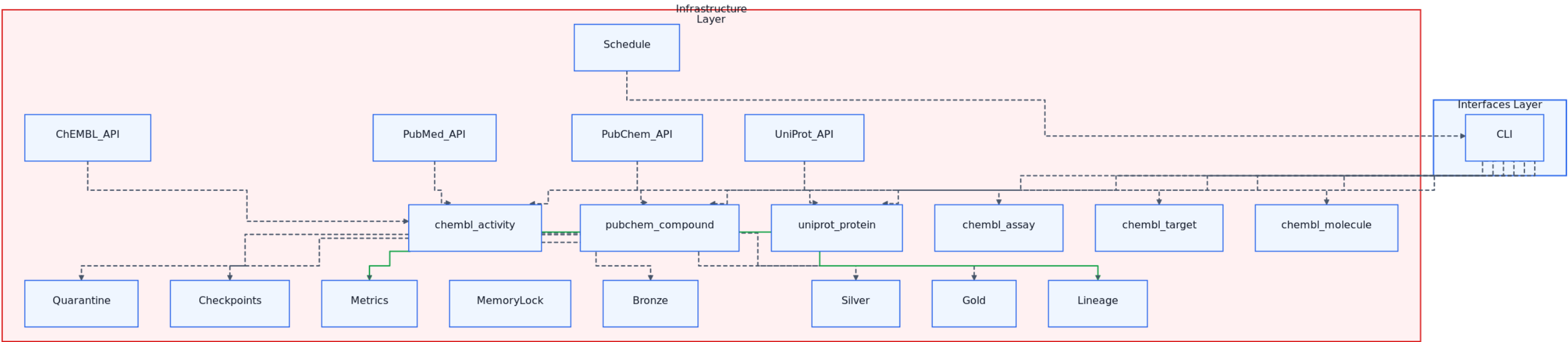
12-local-deployment-architecture-infra
