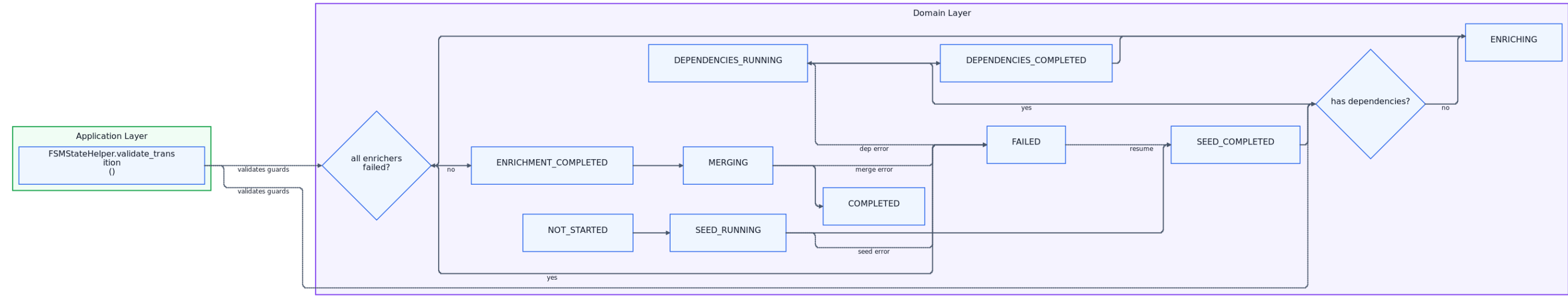
48-composite-phase-lifecycle-domain
