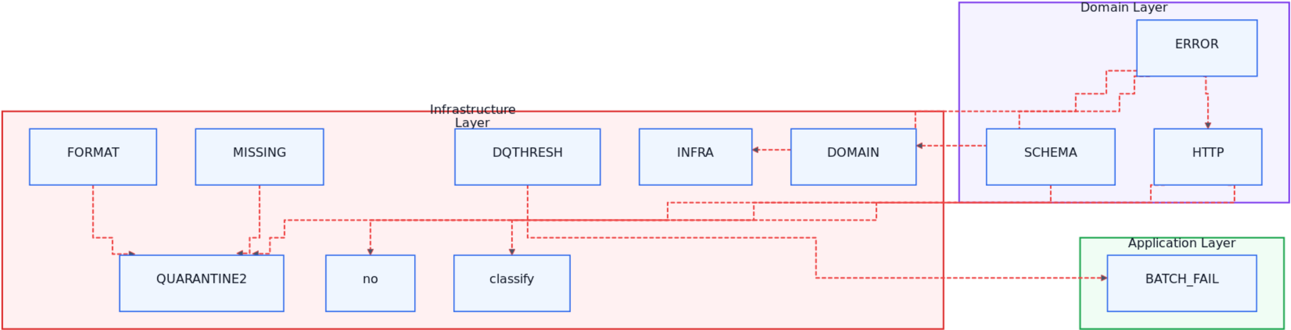
41-error-classification-tree-dataflow
