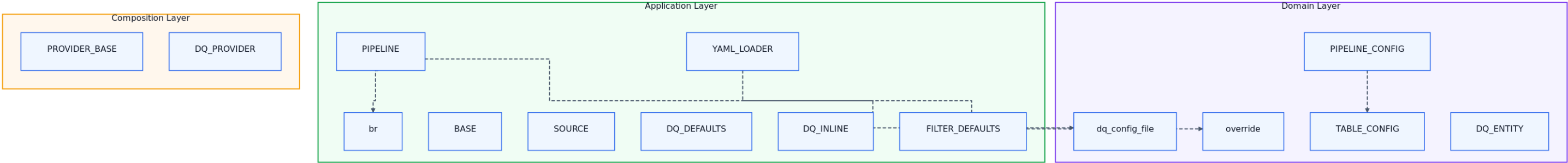
46-yaml-config-resolution-overview
