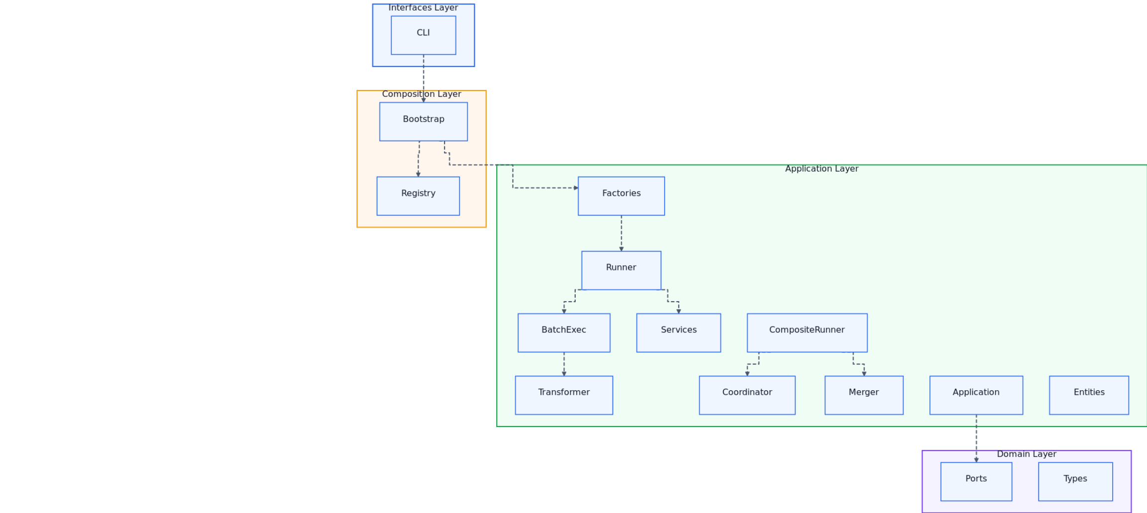
05-layers-interaction-overview
