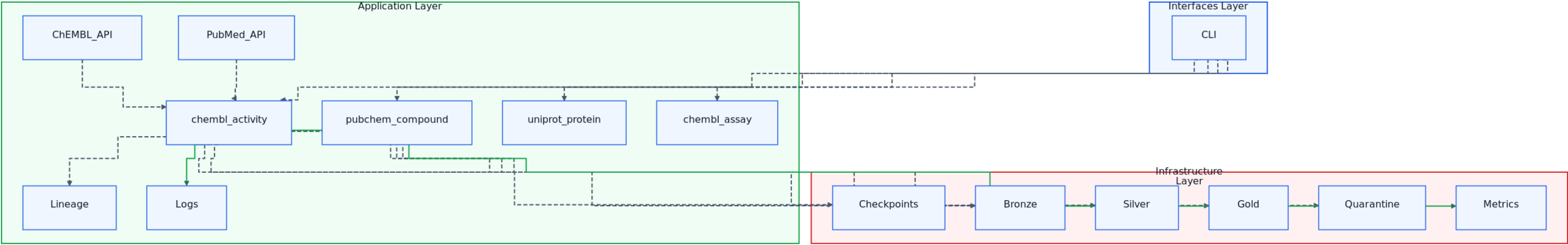
12-local-deployment-architecture-overview
