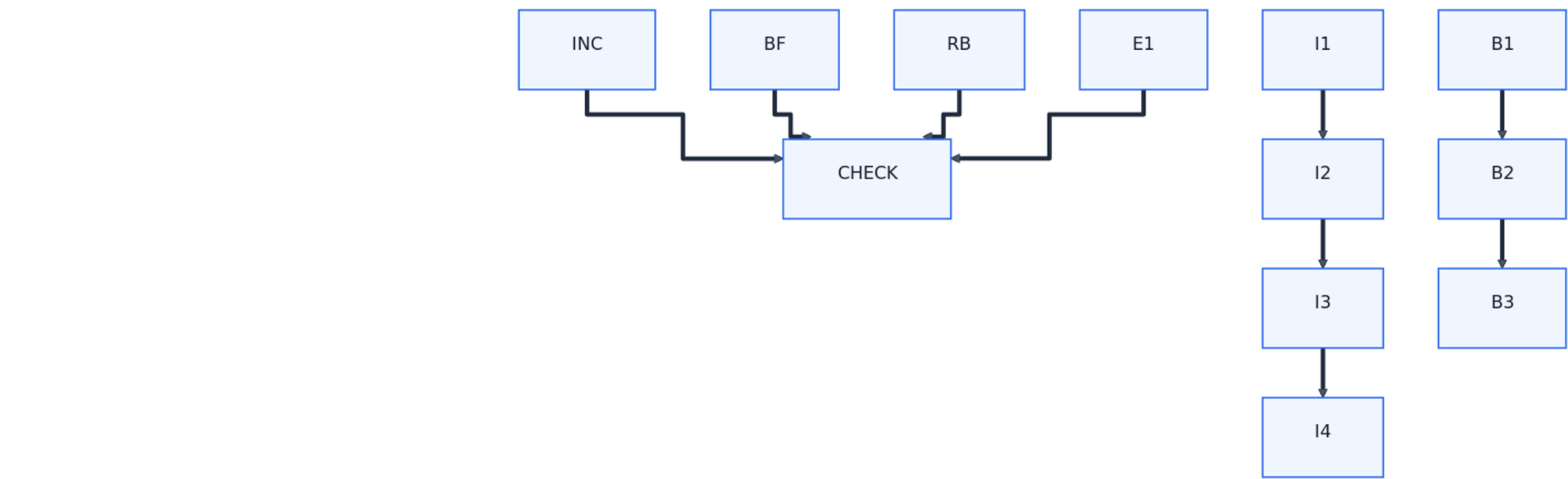
39-medallion-invariants-dataflow
