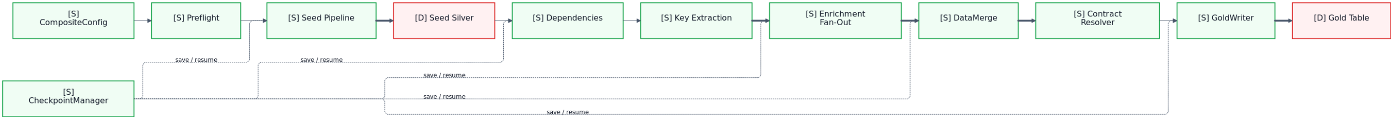
29-composite-pipeline-workflow-overview
