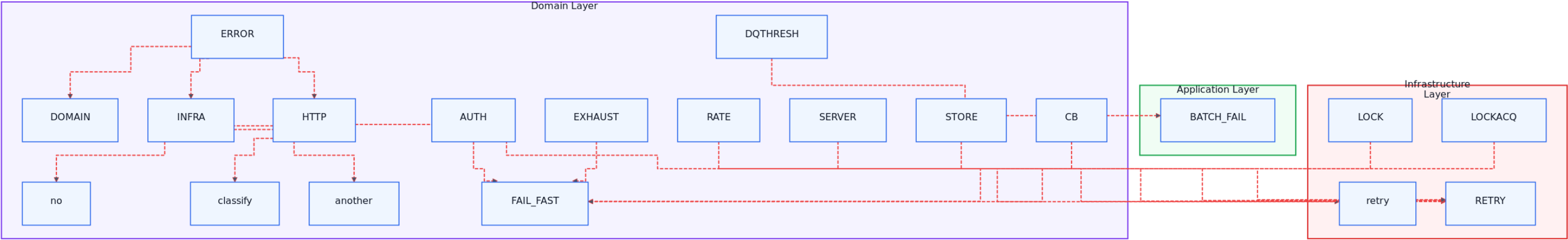
41-error-classification-tree-domain
