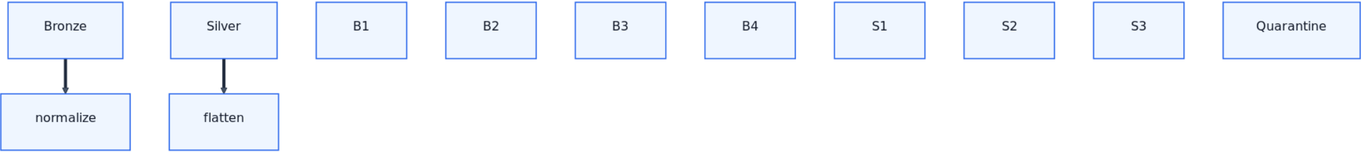
02-medallion-dataflow
