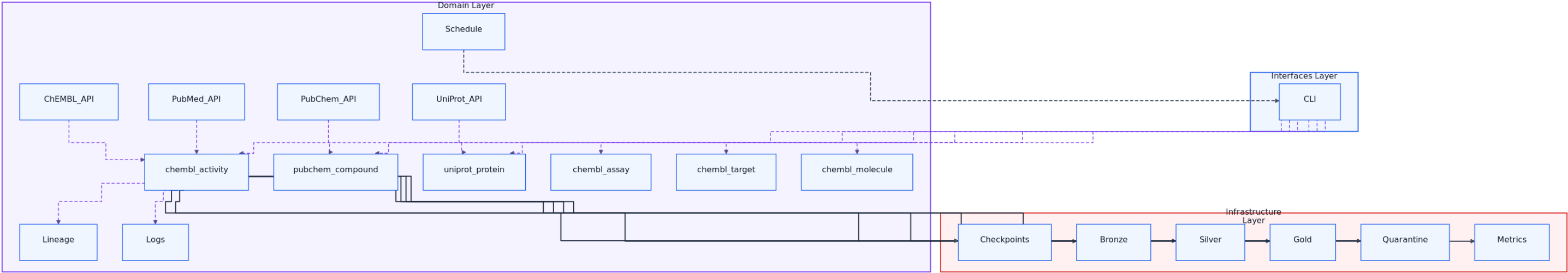
12-local-deployment-architecture-domain
