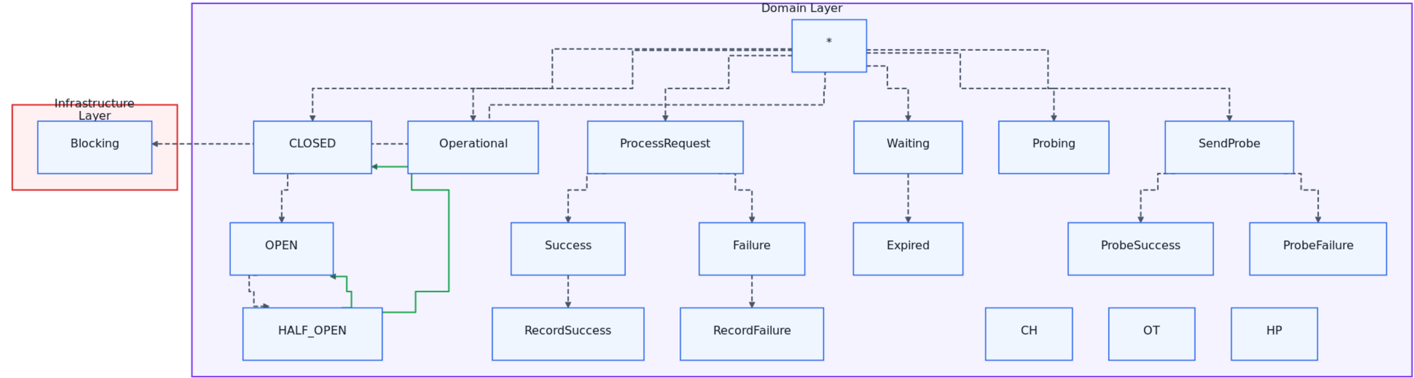
07-circuit-breaker-states-domain
