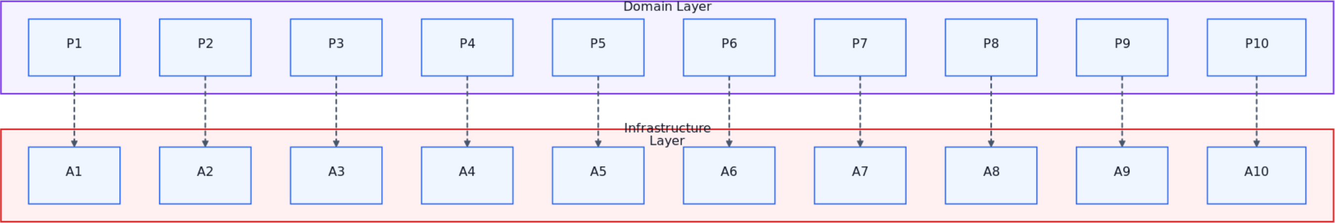
30-port-adapter-mapping-infra
