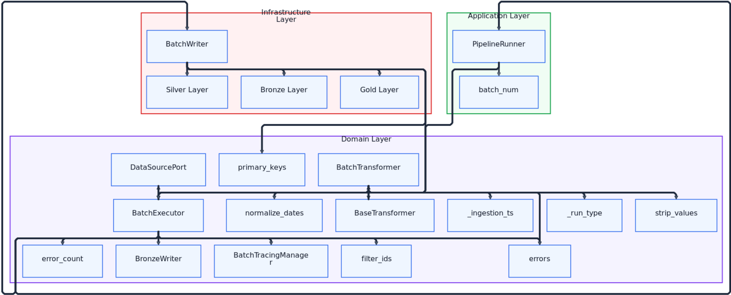
34-batch-processing-flow-domain
