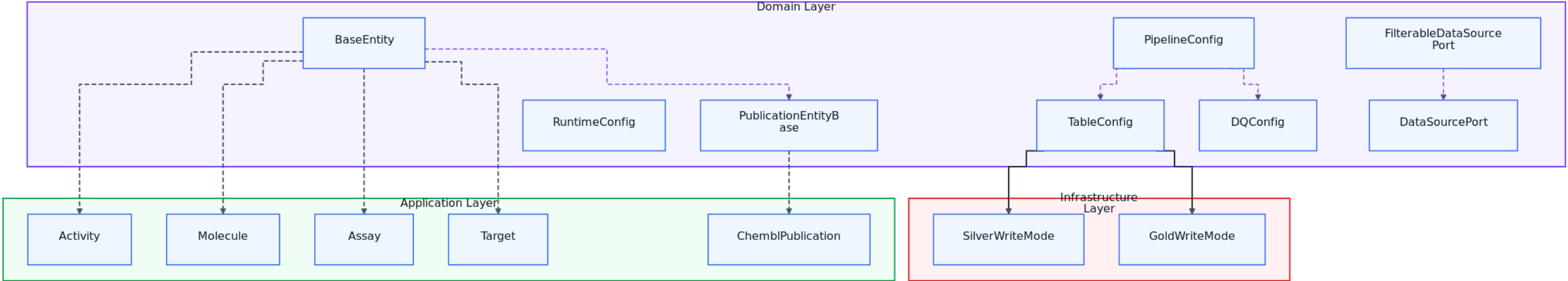
04-domain-layer-class-diagram-overview
