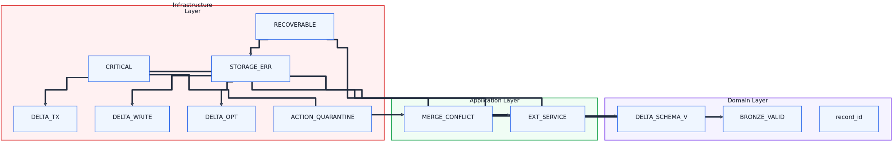
50-exception-hierarchy-dataflow
