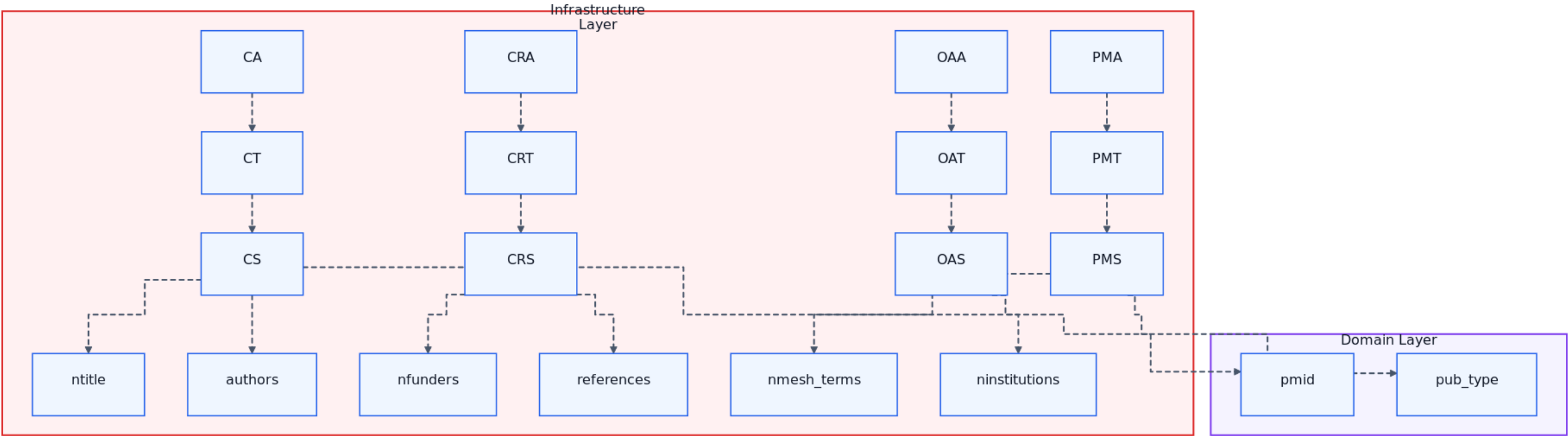
44-cross-provider-enrichment-infra
