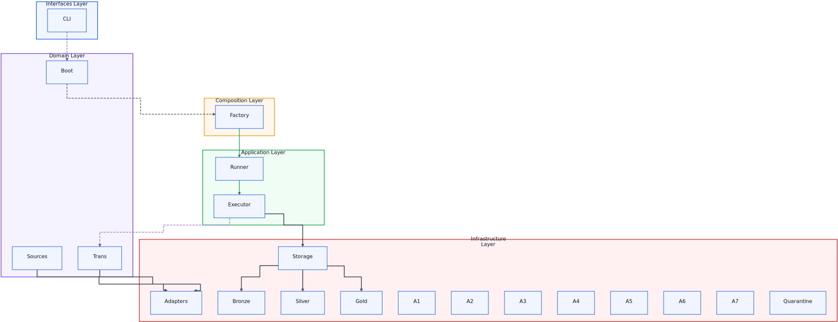
01-high-level-domain
