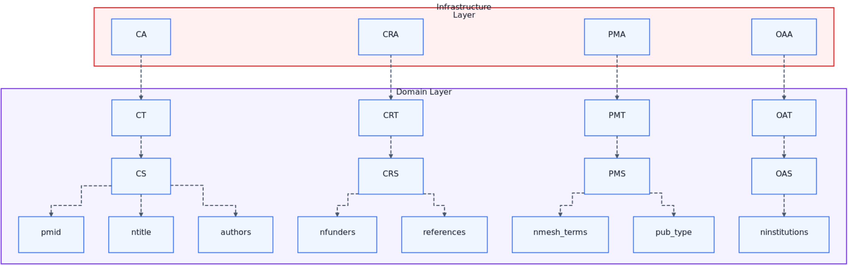
44-cross-provider-enrichment-domain
