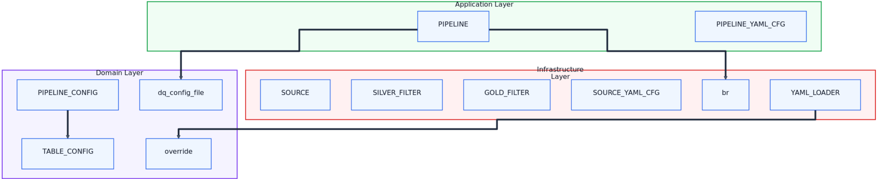
46-yaml-config-resolution-dataflow
