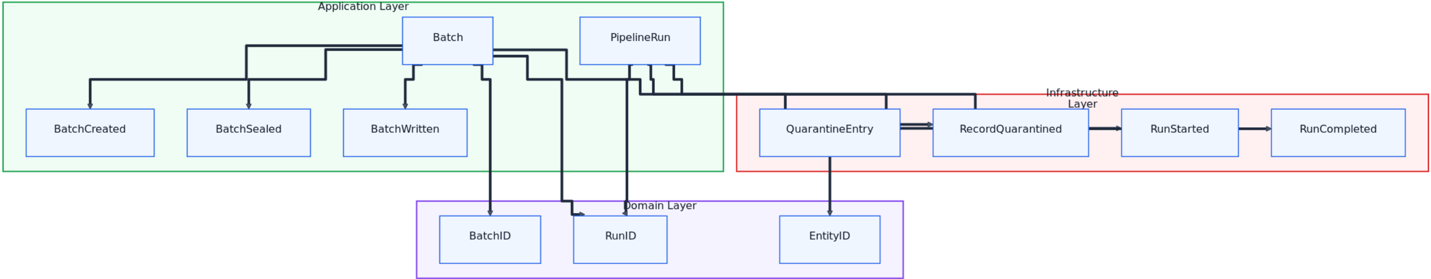
08-domain-ddd-dataflow
