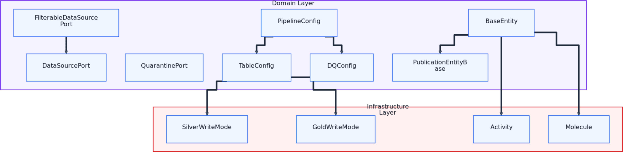
04-domain-layer-class-diagram-dataflow
