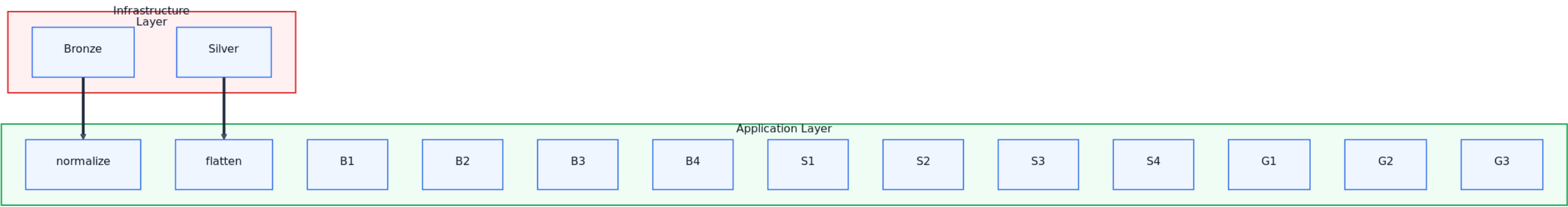
02-medallion-overview
