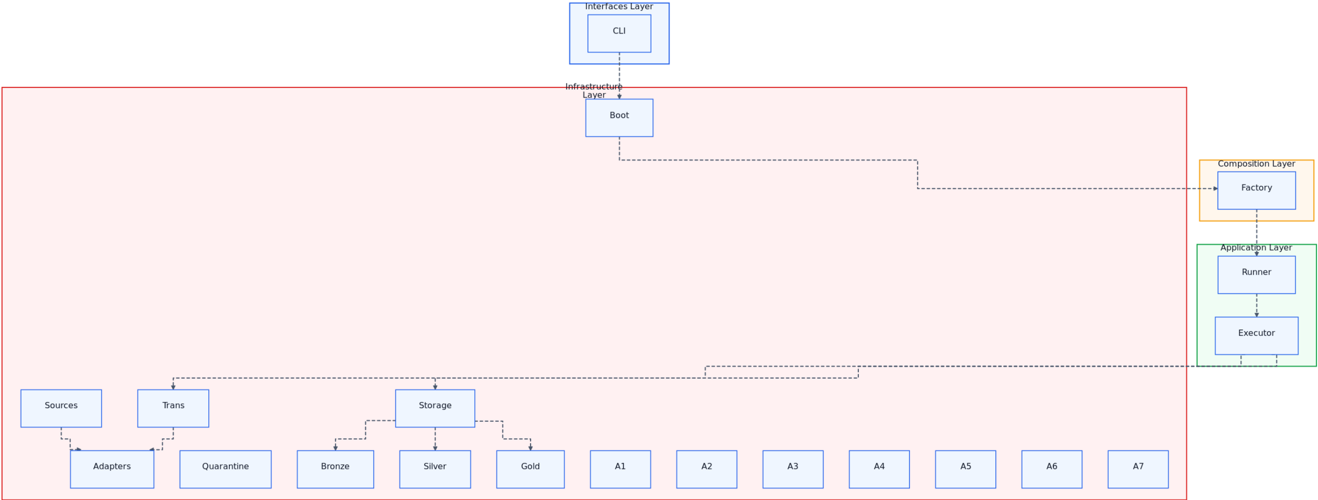
01-high-level-infra
