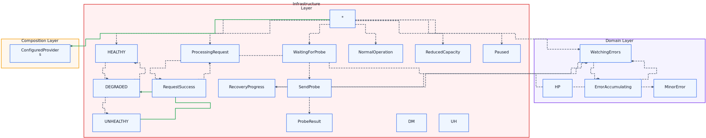
14-provider-health-states-infra
