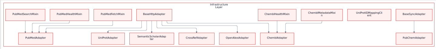
012. architecture/png/05b-adapter-hierarchy-providers.png
