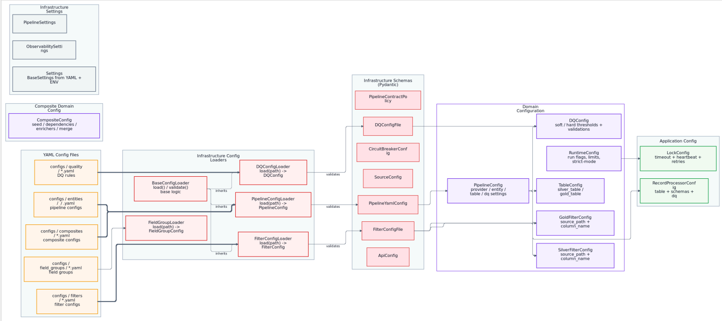
018. architecture/png/11-configuration-system.png
