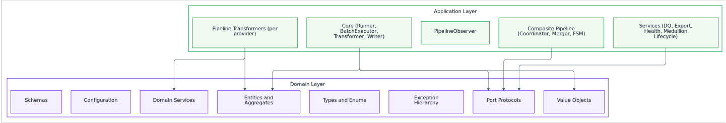
003. architecture/png/01b-hexagonal-domain-app.png
