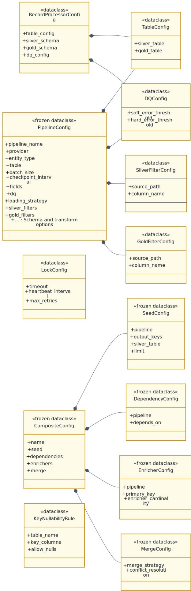
06-config-classes
