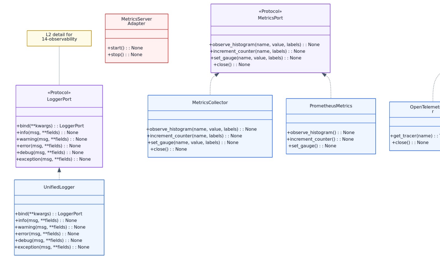
14a-observability-method-catalog
