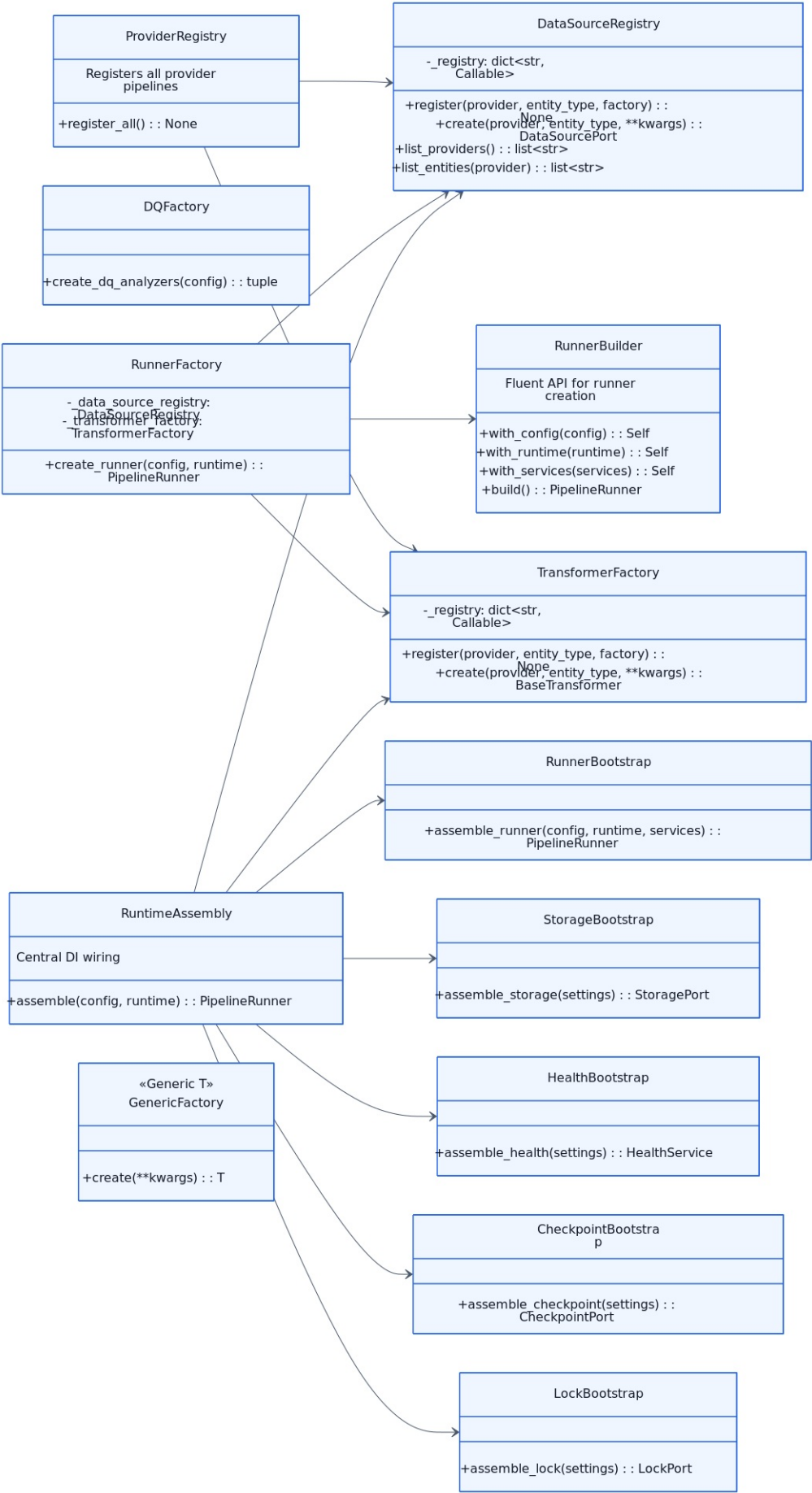
16-factories-bootstrap
