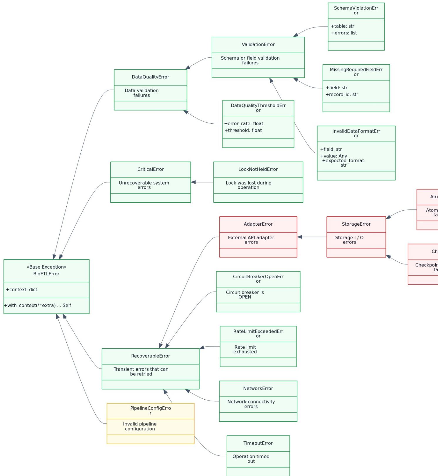
05-exceptions
