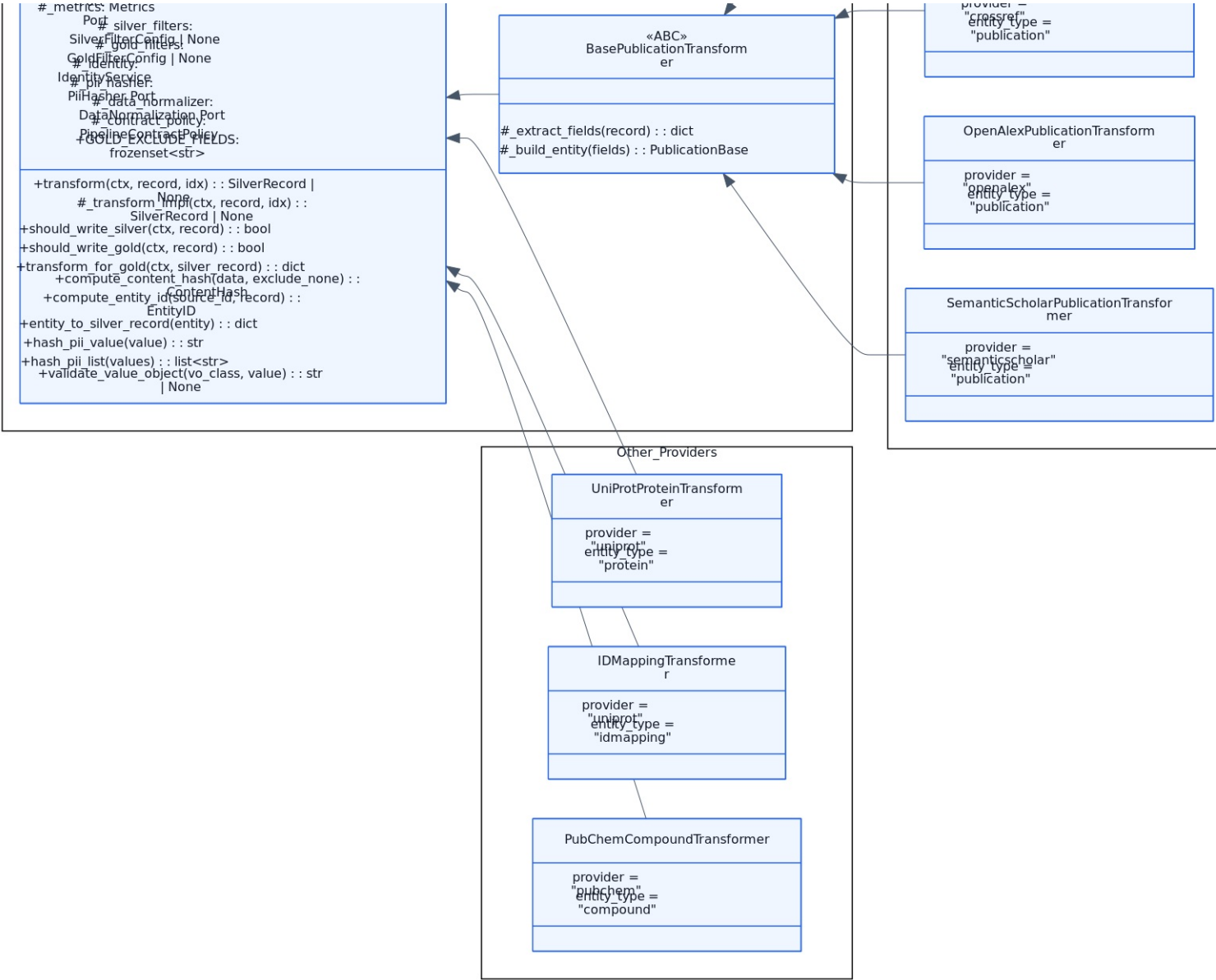
09-transformers
