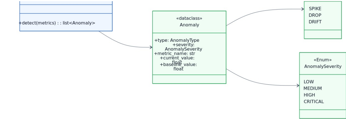
14-observability
