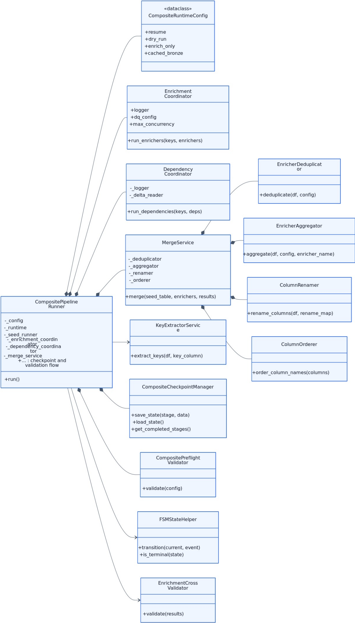
12-composite-pipeline
