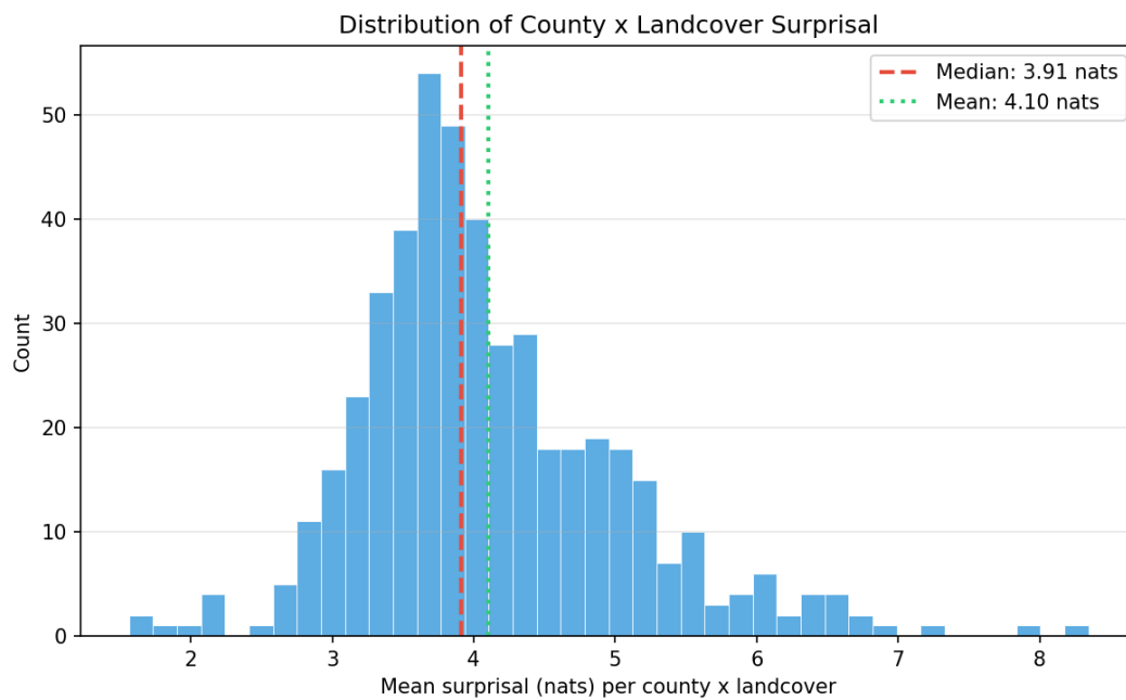
(b) Distribution of mean surprisal across county \times landcover groups. The right tail highlights a small number of unusually high surprisal groups.
