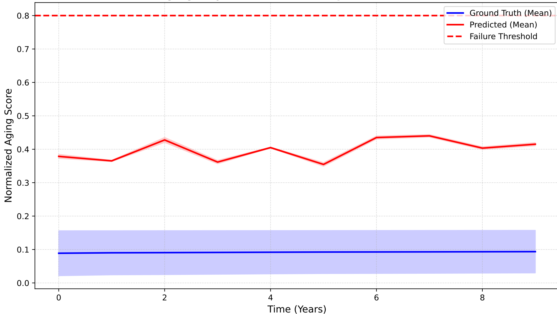
Aging Trajectories Over Component Lifetime
