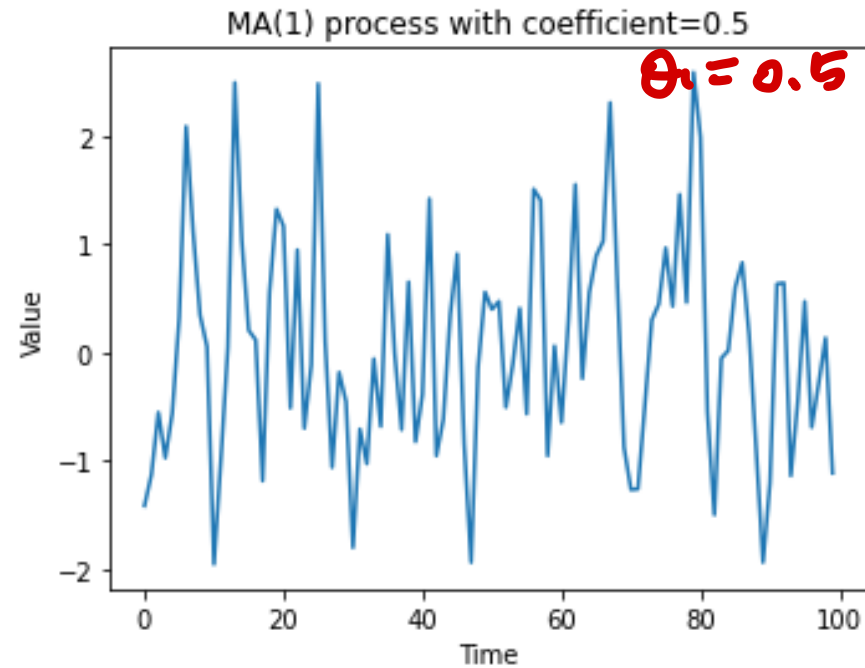
Figure: AR(1) and MA(1) processes
