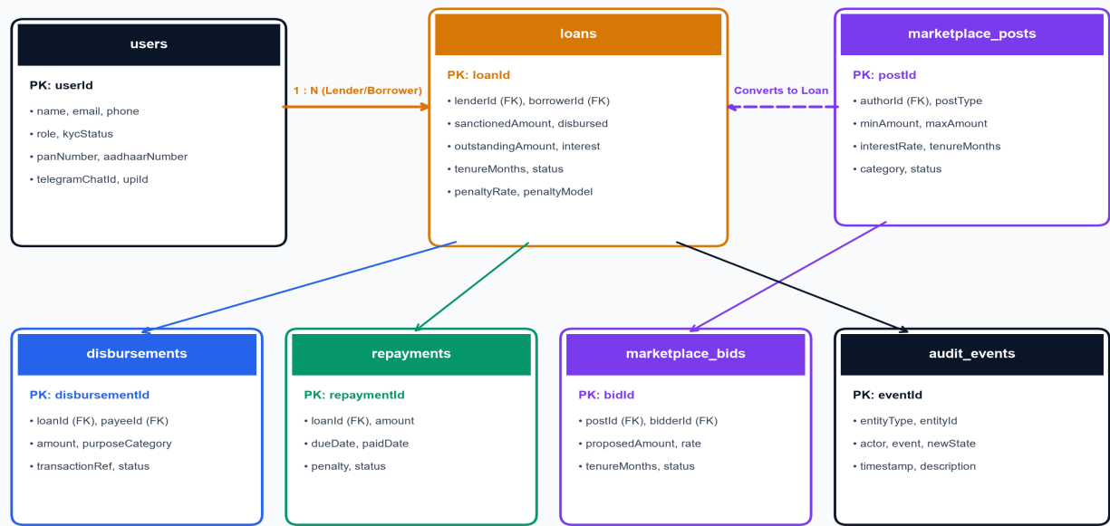
LOANZO DATABASE ENTITY-RELATIONSHIP DIAGRAM (ROOM v11)
