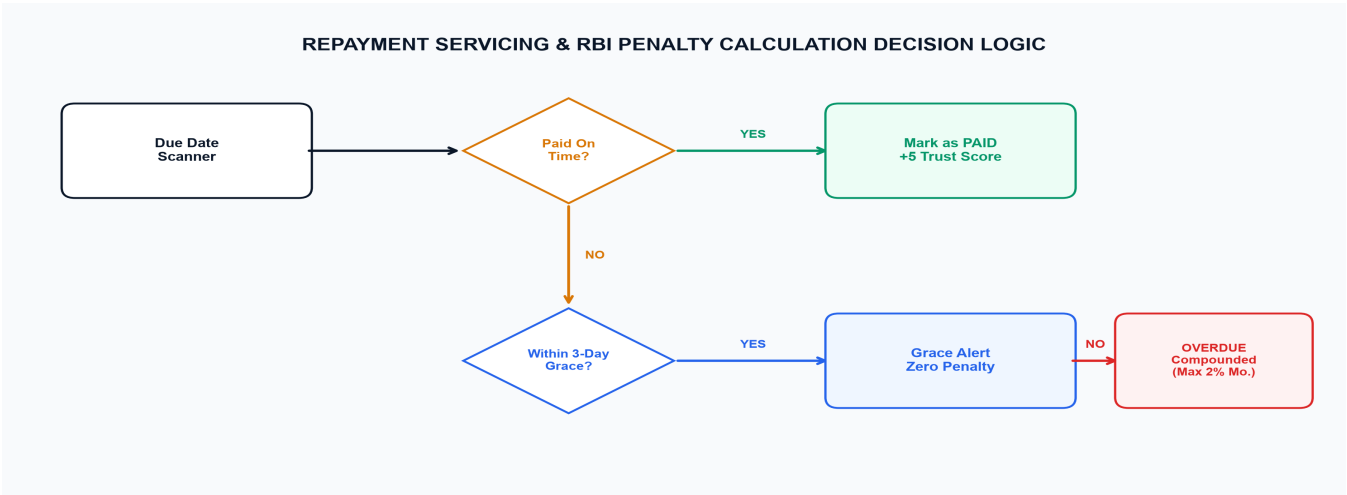
Figure 10.2: Compound Penalty Engine Decision Tree (RBI 2% Cap)
