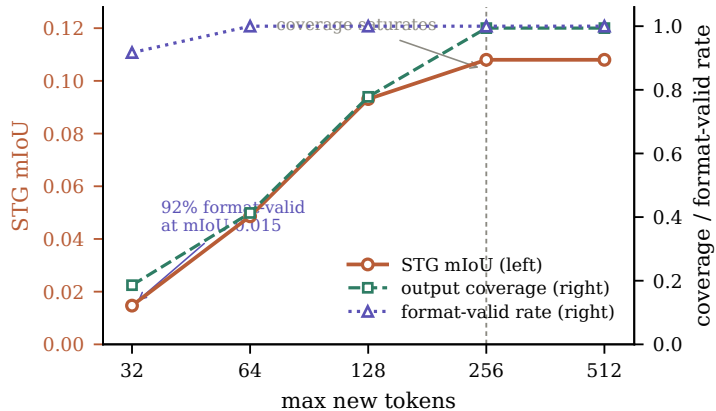
(a) STG performance is bounded by output budget
