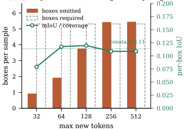
(b) Quality is constant; coverage is everything
