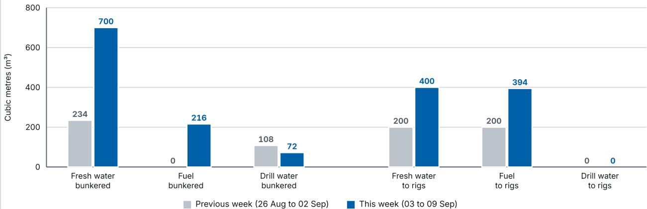
Fluids and bulk managed (1,782 m³ this week, 742 m³ previous week)
