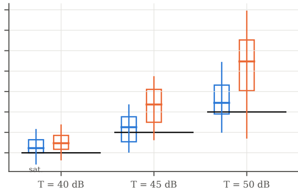
x264 medium
