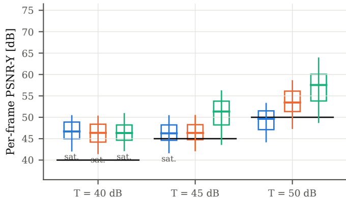
x264 ultrafast
