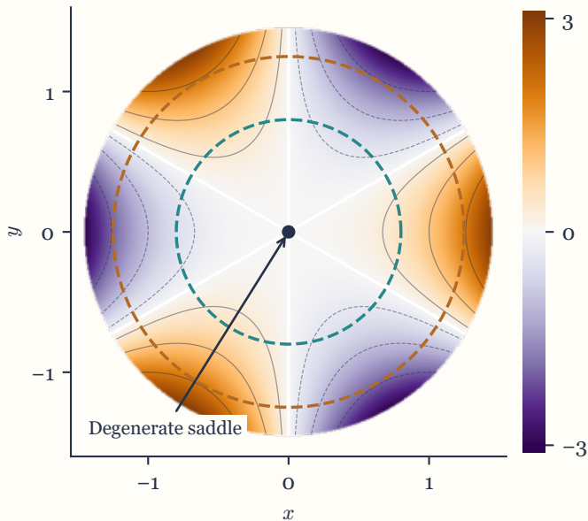
A Three hills, three valleys
