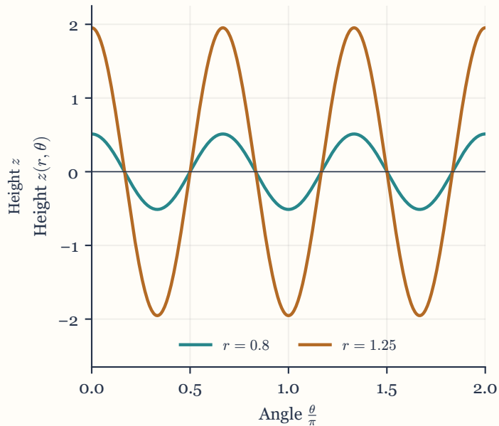
B Walk around the saddle
