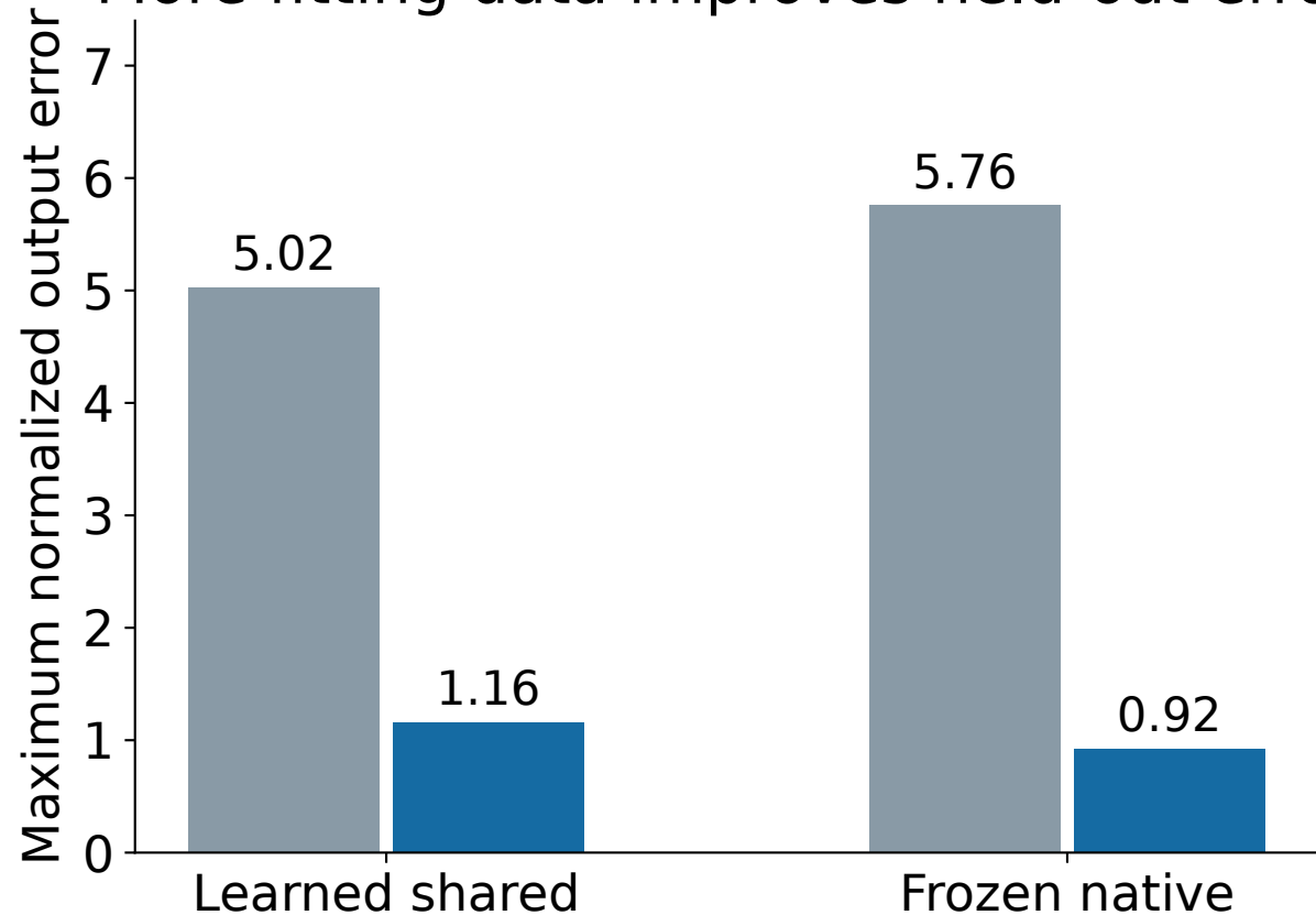
More fitting data improves held-out error
