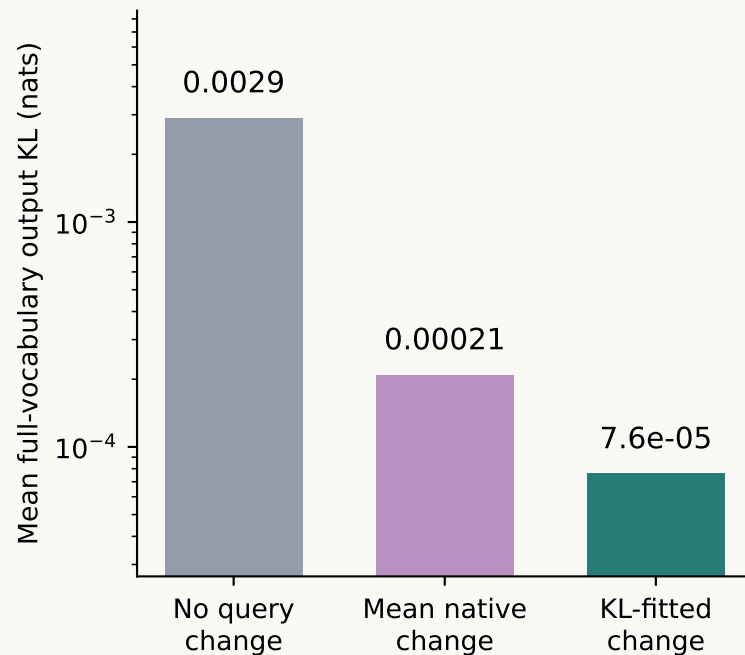
Downstream prediction Four selected heads, changed together
