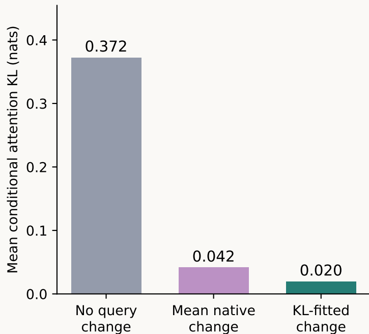
Routing prediction All 448 heads
