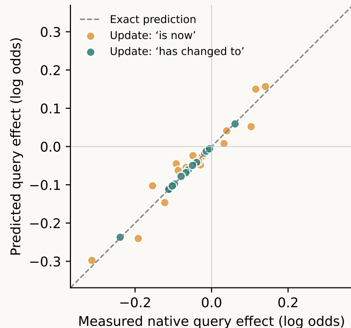
Effect on the answer preference Updated value versus original value
