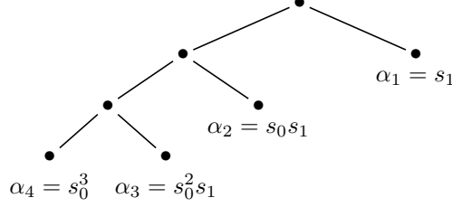
FIGURE 3. The left comb \mathcal{C}_4 : every left child is subdivided. Reading left edges as s_0 and right edges as s_1 , each leaf spells its word along the path from the root; the ordering lists the leaves by depth, with the leftmost branch last.
