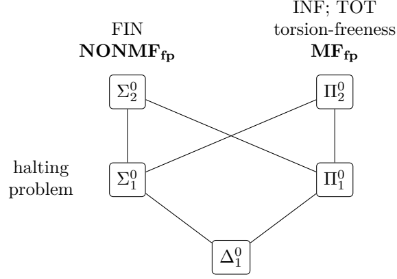
Figure 1: The arithmetical hierarchy. Lines indicate inclusions, and each listed problem is complete at its level. The two sets of Theorem A appear in bold: \text{MF}_{\text{fp}} \in \Pi^0_2 by the finite certificates of Section 3, and the family \hat{R}_e of Section 5 reduces INF to \text{MF}_{\text{fp}} and FIN to \text{NONMF}_{\text{fp}} .
