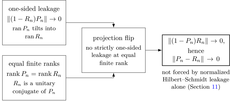
FIGURE 2. Equal-rank reversal. One-sided spectral leakage, together with equality of the two finite ranks, forces the reverse leakage — bounded by \eta/\sqrt{1-\eta^2} — and hence convergence of the two projections. The reversal uses equality of the finite coordinate ranks; normalized Hilbert–Schmidt-small leakage alone neither controls those ranks nor yields the reverse operator-norm estimate (Section 11).
