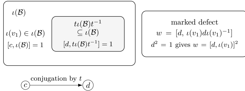
FIGURE 1. The marked-compression pattern. Conjugation by t carries the image of the literal base into itself. It sends c to d = tct^{-1} , which centralizes that compressed copy. Only the one-sided inclusion is used; no injectivity or strict containment is asserted.
