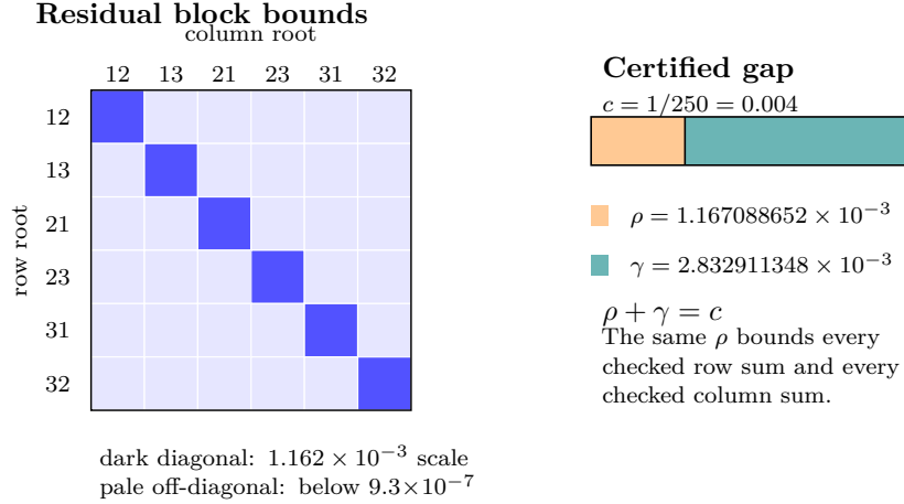
FIGURE 2. Exact Hodge-certificate scale. The residual grid distinguishes the diagonal and off-diagonal block bounds; the separate bar partitions c = 1/250 into the certified residual radius \rho and positive gap \gamma = c - \rho .
