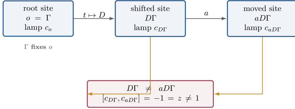
FIGURE 2. The Clifford witness for w \neq 1 . The base fixes the root lamp, while the proper doubling shift creates two distinct Clifford sites whose commutator is the central sign.
