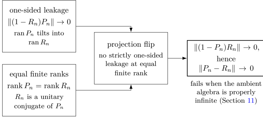
FIGURE 3. Equal-rank reversal. One-sided spectral leakage, together with equality of the two finite ranks, forces the reverse leakage — bounded by \varepsilon'/\sqrt{1 - (\varepsilon')^2} — and hence convergence of the two projections. In a properly infinite algebra, nested unitarily equivalent projections need not coincide, which is why the argument does not transfer to tracial ultra-products (Section 11).
