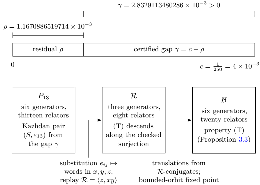
FIGURE 2. Exact certificate and descent. Top: the spectral floor c = 1/250 of (8) splits into the certified residual radius \rho of (9) and the positive gap \gamma = c - \rho of (10); the partition is drawn to scale. Bottom: property (T) travels from P_{13} through the checked surjection onto \mathcal{R} , then to the literal base \mathcal{B} by the fixed-point argument for the translations (Proposition 3.3).
