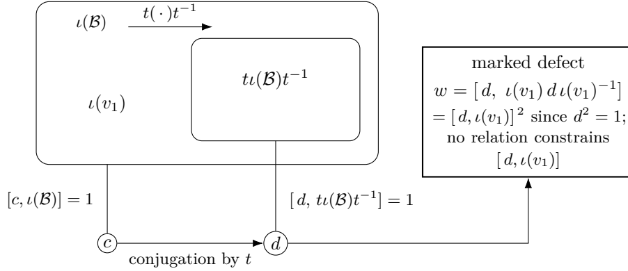
FIGURE 1. The marked-compression pattern. Conjugation by t carries the image of the literal base into itself. It sends c to d = tct^{-1} : the relations tie c to all of \iota(\mathcal{B}) but tie d only to the compressed copy, and the marked word w records the unconstrained commutation with \iota(v_1) . Only the one-sided inclusion is used; no injectivity or strict containment is asserted.
