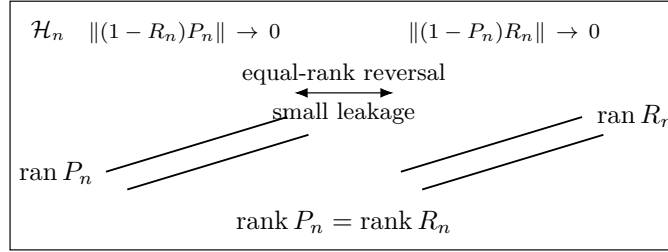
FIGURE 4. Finite-dimensional reversal. One-sided spectral leakage and equality of ranks control the complementary block in the reverse direction; together the two estimates force \|P_n - R_n\| \rightarrow 0 . The drawn planes are schematic ranges inside the common finite-dimensional space \mathcal{H}_n .
