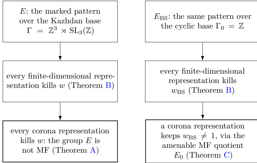
FIGURE 4. The cyclic-base comparison. The finite-dimensional obstruction does not see the base, while the corona conclusion holds exactly on the side where property (T) supplies uniform finite-stage spectral pinning.
