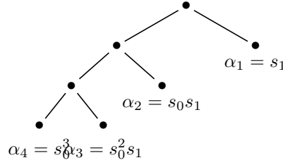
FIGURE 3. The left comb \mathcal{C}_4 : every left child is subdivided. Reading left edges as s_0 and right edges as s_1 , each leaf spells its word along the path from the root; the ordering lists the leaves by depth, with the leftmost branch last.
