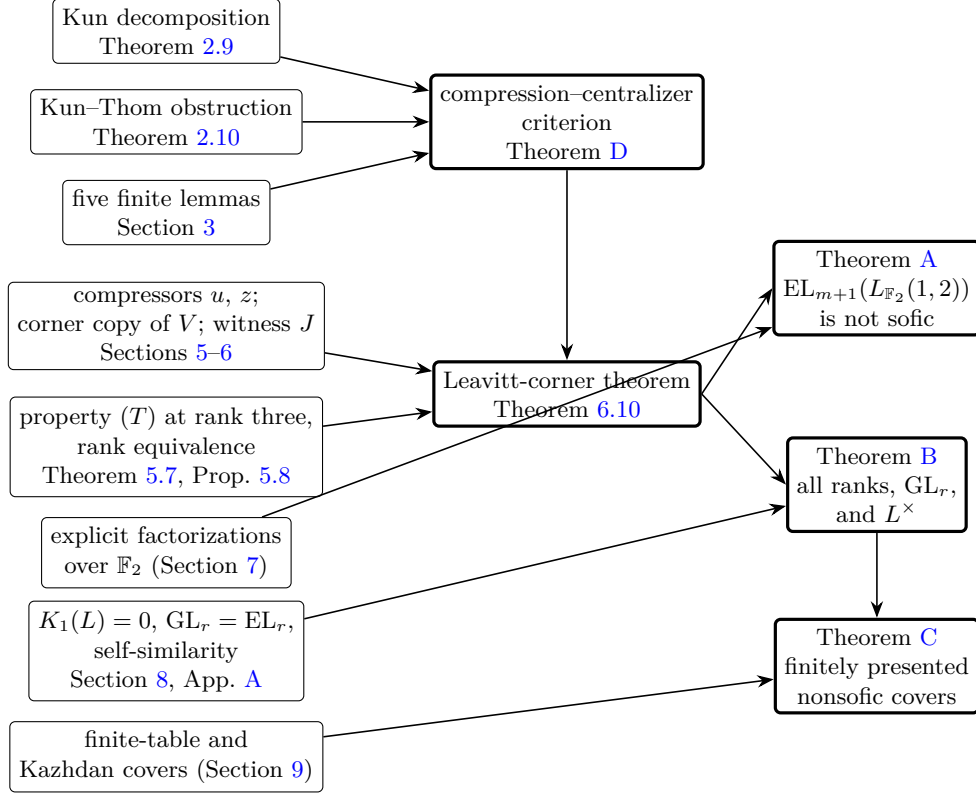
FIGURE 1. The architecture of the proof. The analytic layer (top left) produces the criterion; the algebraic layer (middle left) realizes its hypotheses over any ring carrying a binary Leavitt family; the memberships are discharged twice, explicitly in characteristic two and K -theoretically over every finite field; and the finite-table layer converts nonsoficity into finitely presented covers.
