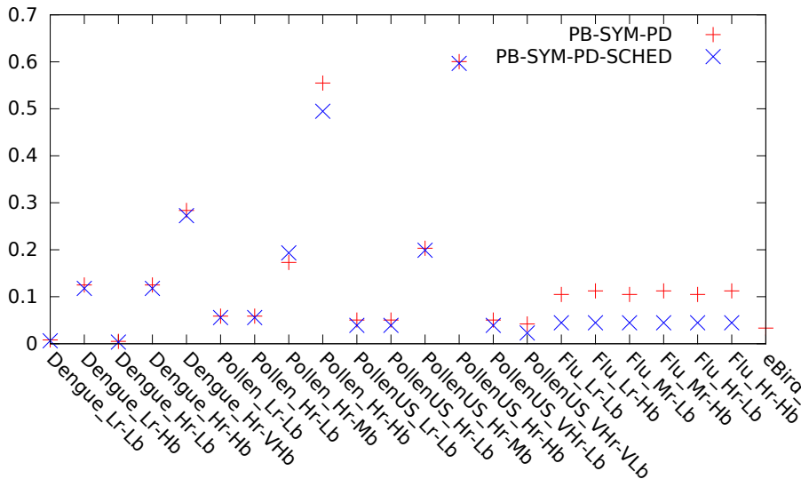
Relative length of the critical path
