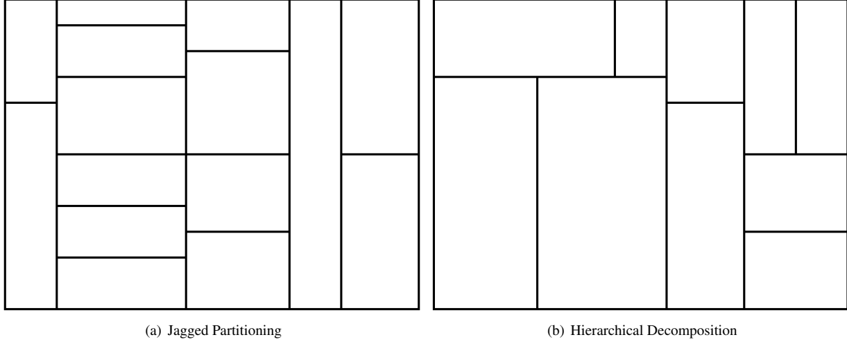
Figure 20: 2D representation of the two types of decomposition addressed in this paper. Jagged partitioning form vertical stripes which are then partitioned horizontally. Hierarchical decomposition are defined recursively by cutting the domain in a grid aligned manner.
