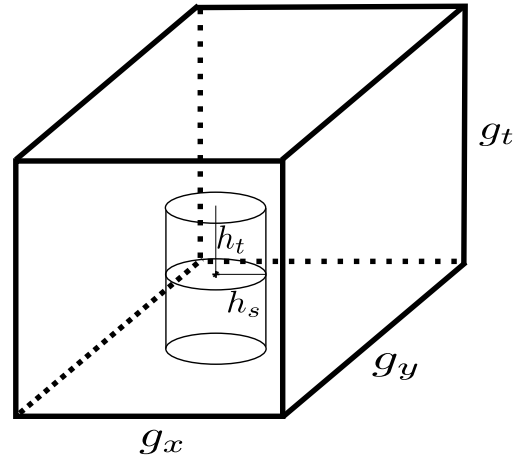
Figure 17: The computation of STKDE happens in a domain space of size g_x, g_y, g_t . Each point impacts the neighboring space at a distance h_s in space and h_t in time; forming a cylinder of diameter 2h_s and of height 2h_t .
