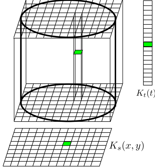
Figure 18: The contribution to the density estimate of each voxel of a cylinder can be decomposed in two terms, one temporally invariant K_s(x, y) and one spatially invariant K_t(t) .
