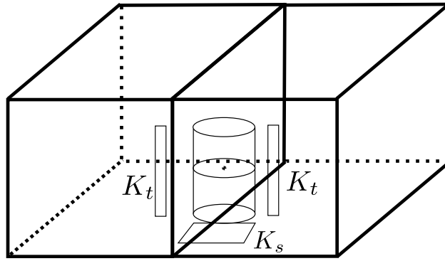
Figure 19: When a cylinder is split among two subdomains, PB-SYM-DD causes an overhead because one of the invariant needs to be recomputed. Here each subdomains compute part of the temporal invariant K_s , but both need to compute the spatial invariant K_t .
