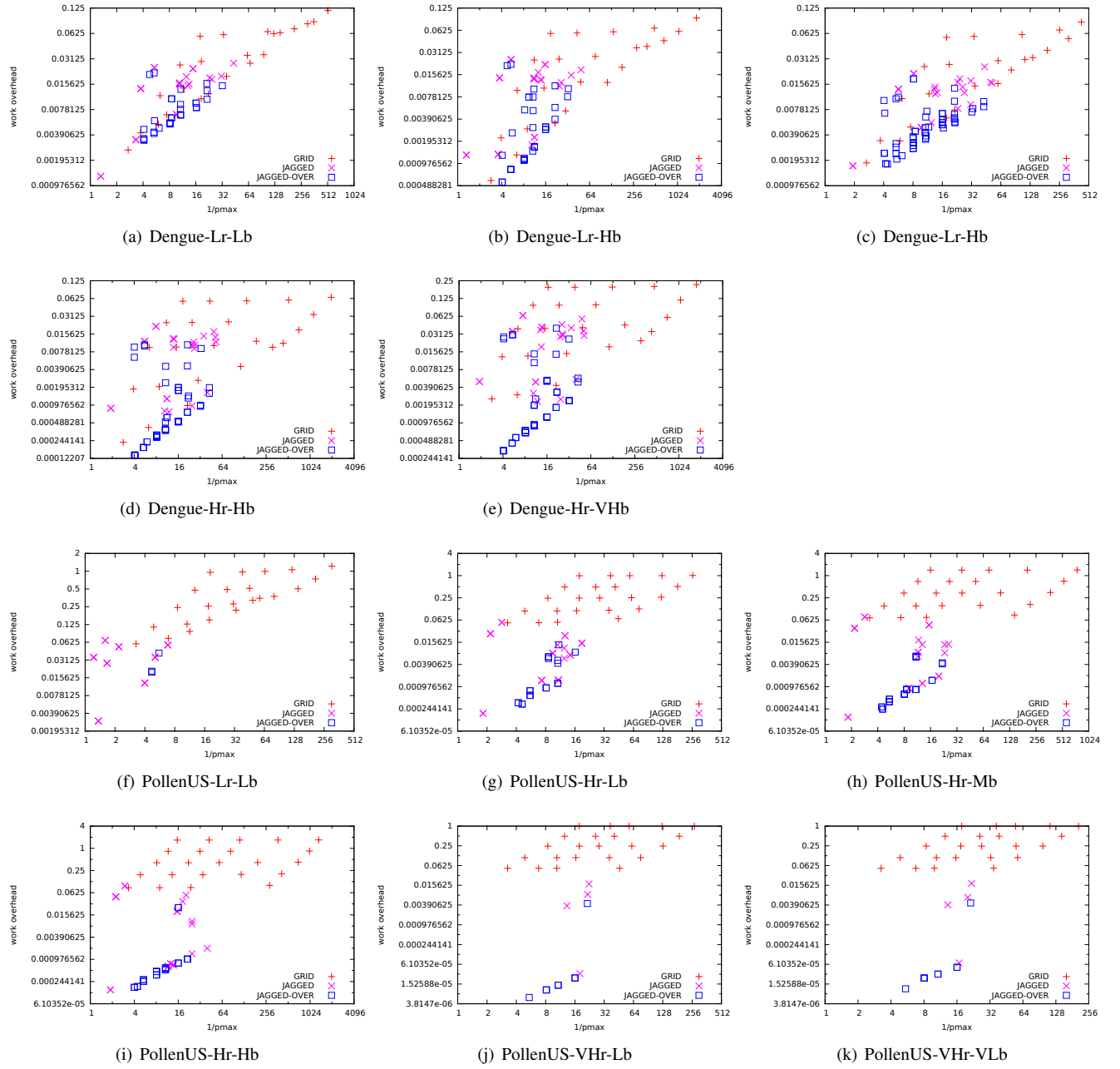
Figure 23: Quality of partitioning generated by Jagged decomposition
