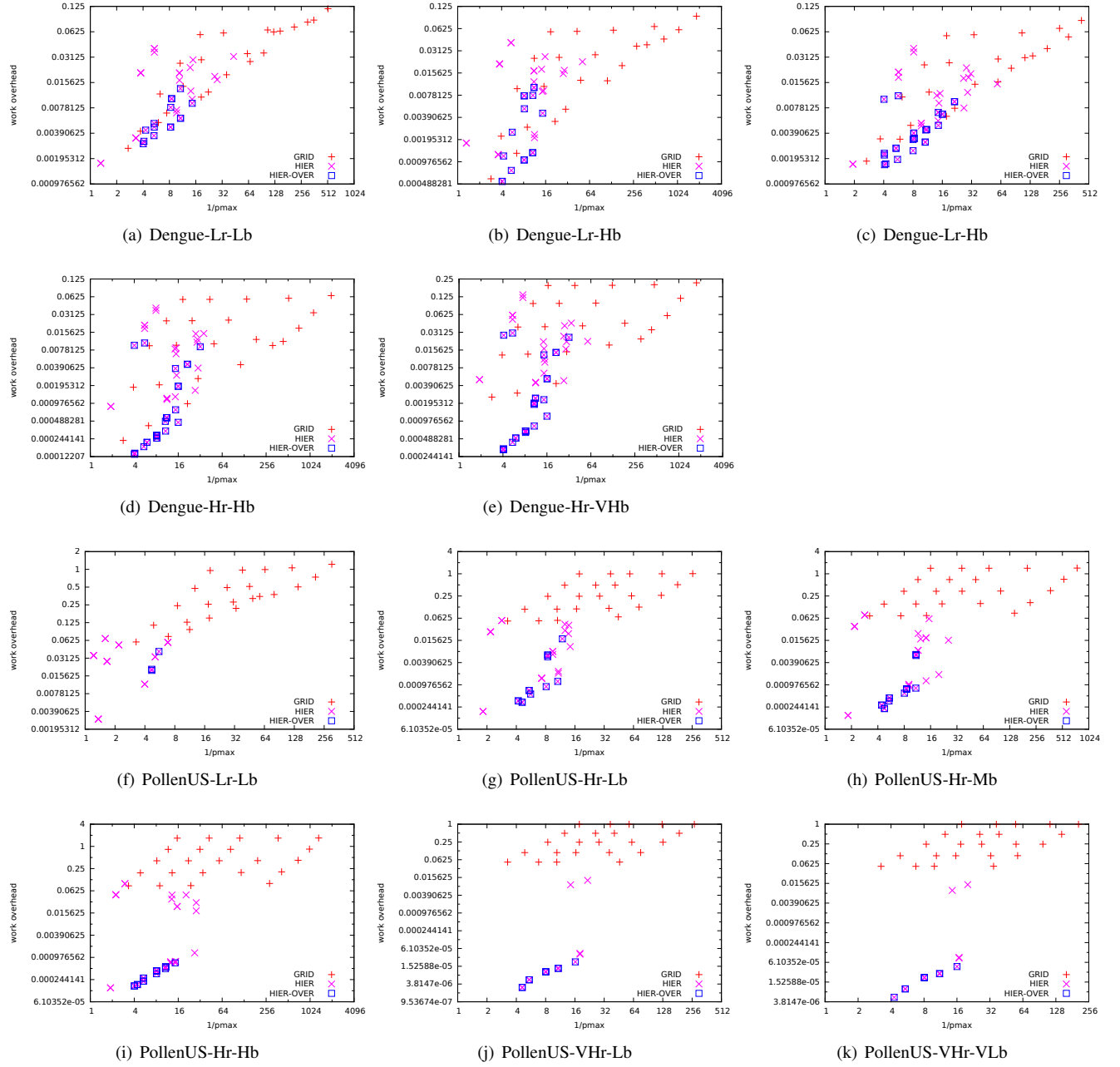
Figure 24: Quality of Partitionings generated by Hierarchical Decomposition
