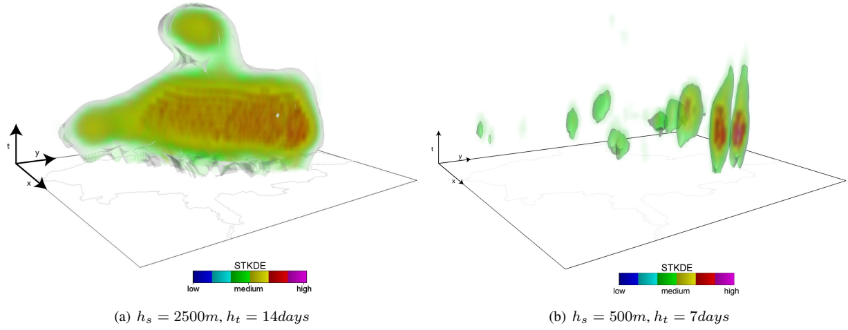
Figure 16: Visualization of Dengue fever cases in Cali, Colombia in 2010 and 2011 for different spatial bandwidth and temporal bandwidth.
