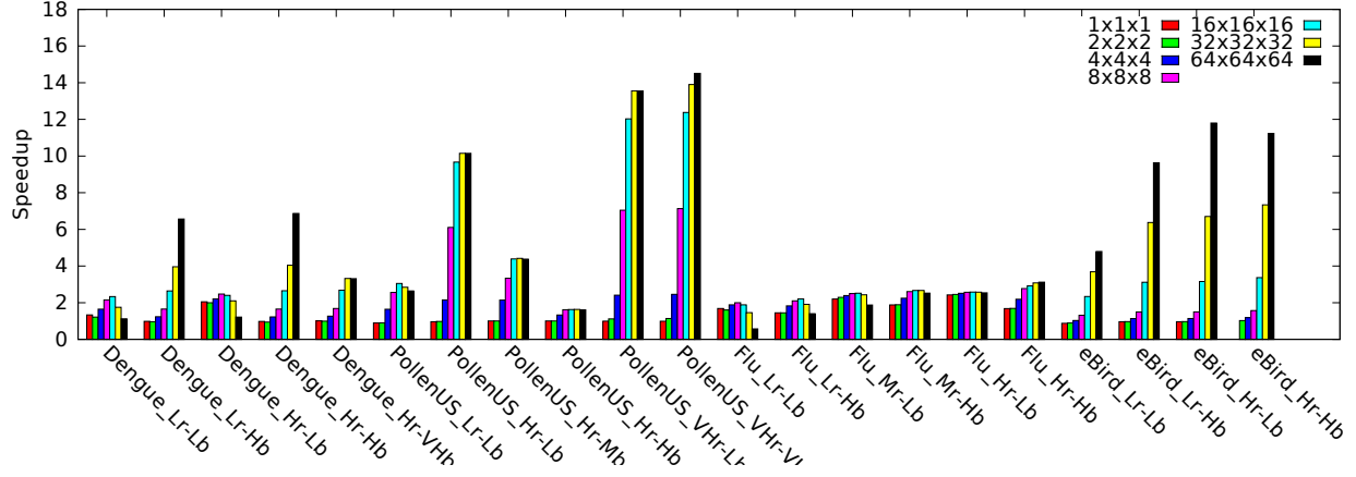
Figure 17: Speedup of PB-SYM-PD using 16 threads. Note that decompositions of subdomain smaller than twice the bandwidths are adjusted.
