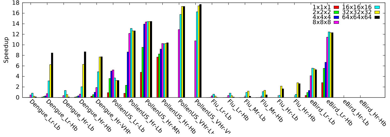
Figure 20: Speedup of PB-SYM-PD-REP using 16 threads for different decompositions. Flu_Hr-Lb and Flu_Hr-Hb run out of memory for small decomposition.
