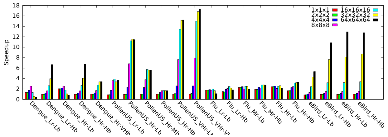
Figure 19: Speedup of PB-SYM-PD-SCHED with 16 threads.
