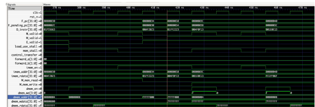
Figure 8 Adjacent-element exchange in the signed sorting loop. Two full-word Port-B write transactions ( dmem_we = 4'hF ) write 0xFFFFFFFF and 0x7FFFFFFF to consecutive local data-BRAM offsets. The two pulses demonstrate that each store is issued once, even though the Memory stage remains occupied by back-to-back stores.
