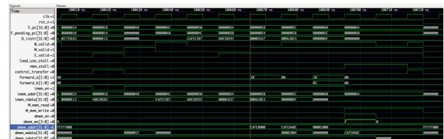
Figure 9 Completion sequence and terminal loop. The instructions LUI , ADDI , LUI , and SW construct 0xCAFEBADE and issue one full-word write at local data-BRAM offset 0x00001000 , corresponding to the reserved DONE location. The following JAL x0, 0 remains in the terminal loop and produces no further data-memory writes.
