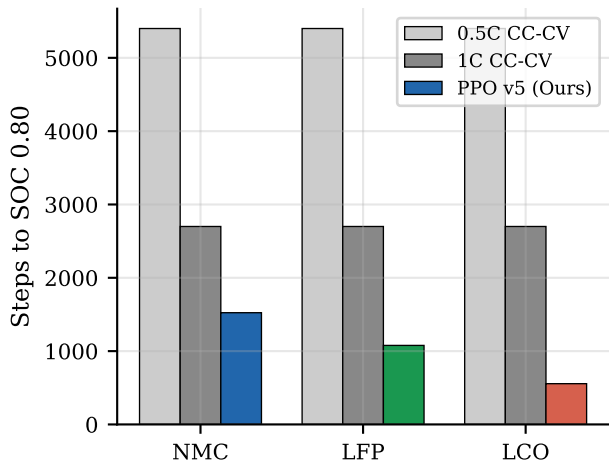
Charging time (5/5 layouts, 100% success)
