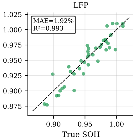
Degradation model fit: predicted vs. true SOH (cell-held-out)
