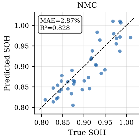
Degradation model fit: predicted vs. true SOH (cell-held-out)
