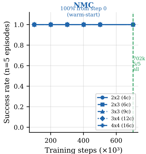
Per-chemistry per-layout success rate — v5 (n_ep=5, warm-start)
