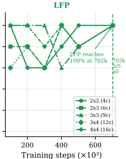
Per-chemistry per-layout success rate — v5 (n_ep=5, warm-start)
