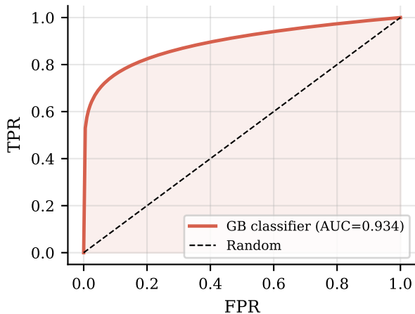
ROC curve
