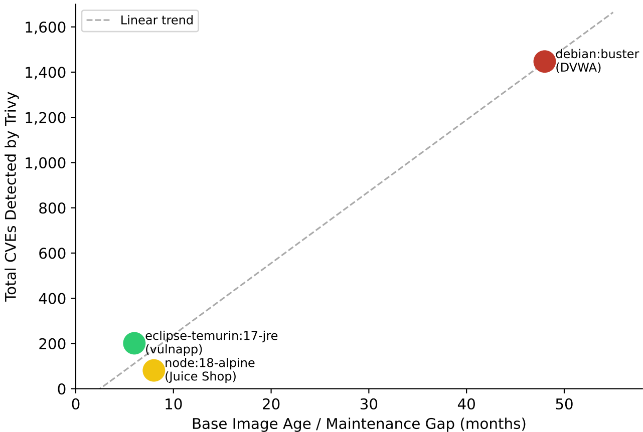
Base-Image Freshness vs. Container Vulnerability Exposure
