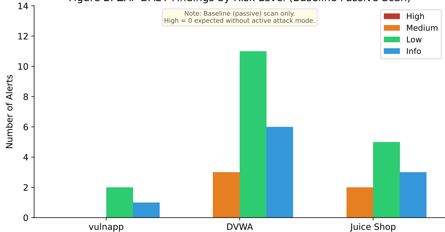
Figure 2: ZAP DAST Findings by Risk Level (Baseline Passive Scan)
