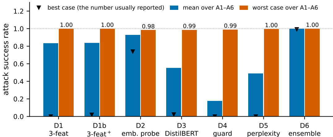
Retrieval-layer defenses at a matched 1% false-positive budget
